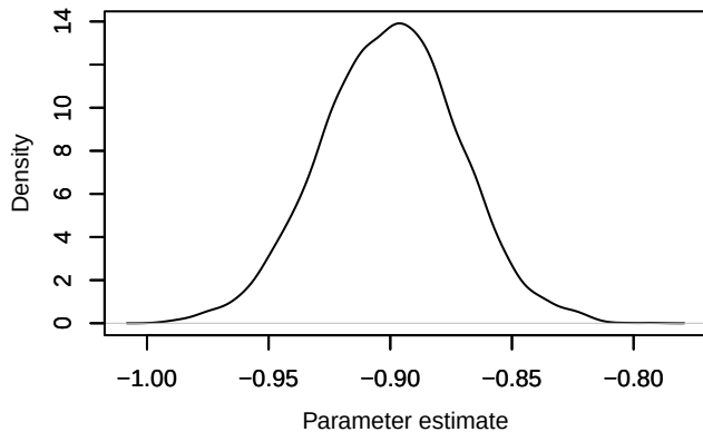
Density – \text{lp}[3, 2]
