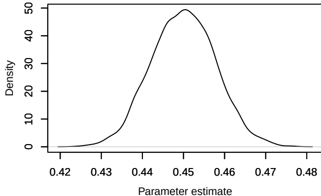
Density – g_eff[2]
