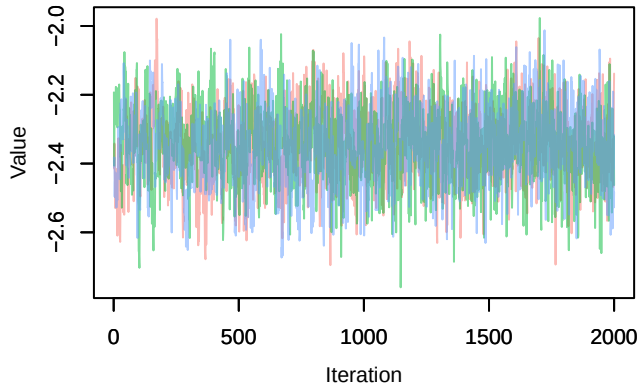
Trace – \text{lp}[4, 1]
