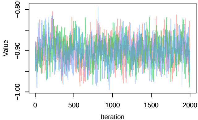
Trace – \text{lp}[3, 2]
