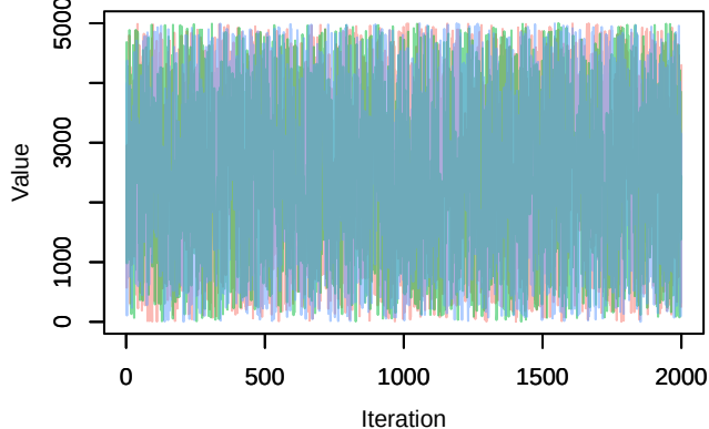
Trace – U0[2, 1]
