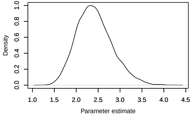
Density – nu[1]
