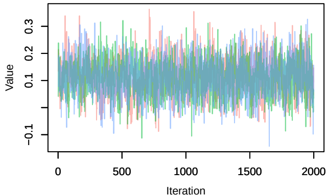
Trace – \text{lp}[7, 1]
