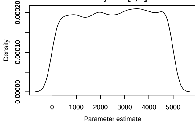
Density – U0[5, 1]
