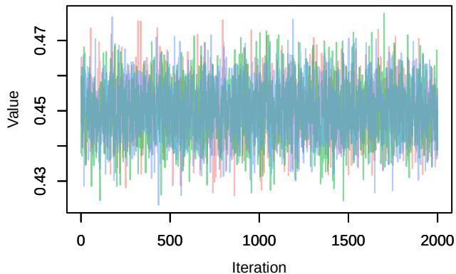
Trace – g_eff[2]
