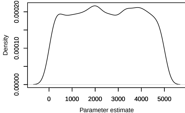
Density – U0[3, 1]
