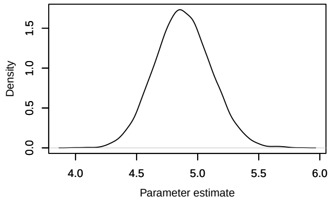
Density – mu_phi[2]
