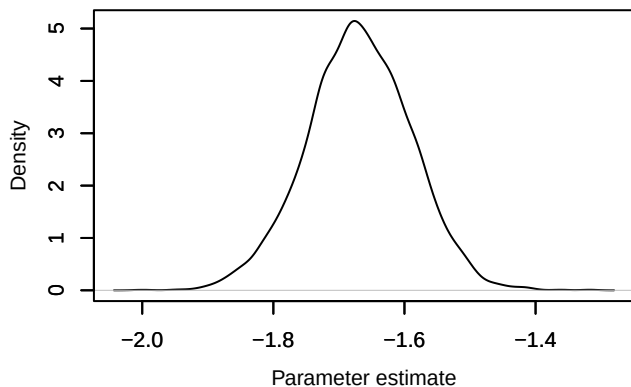
Density – lpsi[2]
