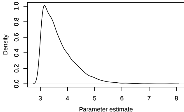
Density – nu[2]
