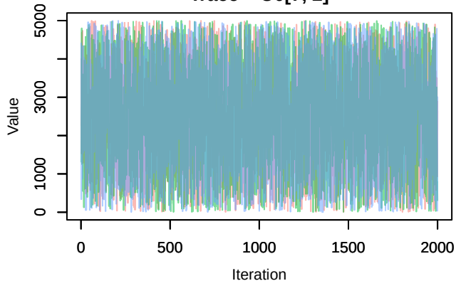
Trace – U0[7, 2]
