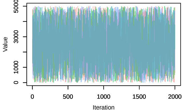
Trace – U0[2, 2]
