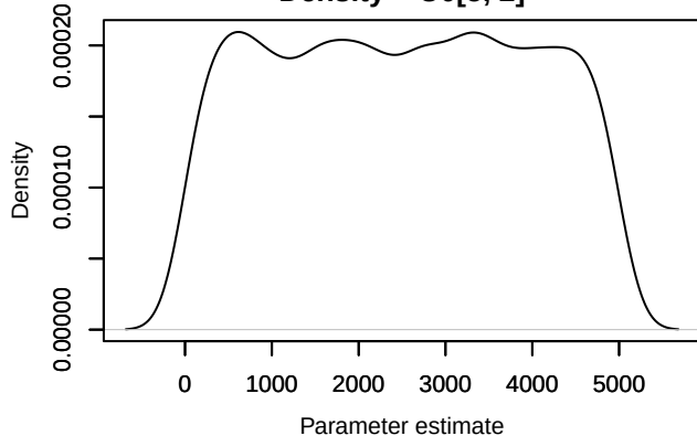
Density – U0[5, 2]
