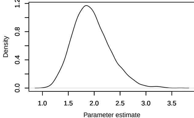
Density – sigma_r[1]
