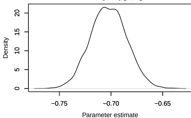
Density – \text{lp}[5, 2]
