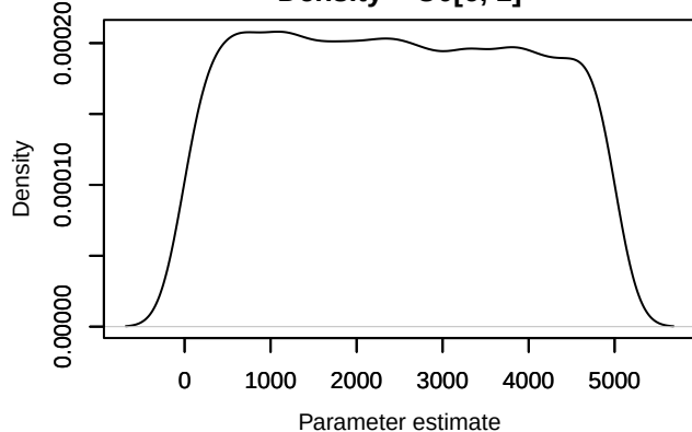
Density – U0[6, 1]
