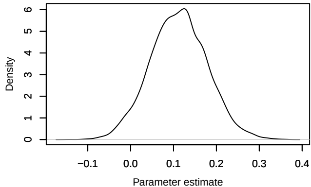
Density – \text{lp}[7, 1]
