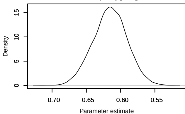
Density – \text{lp}[6, 2]
