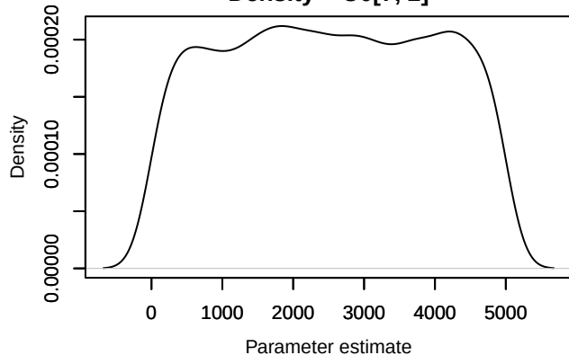
Density – U0[7, 2]
