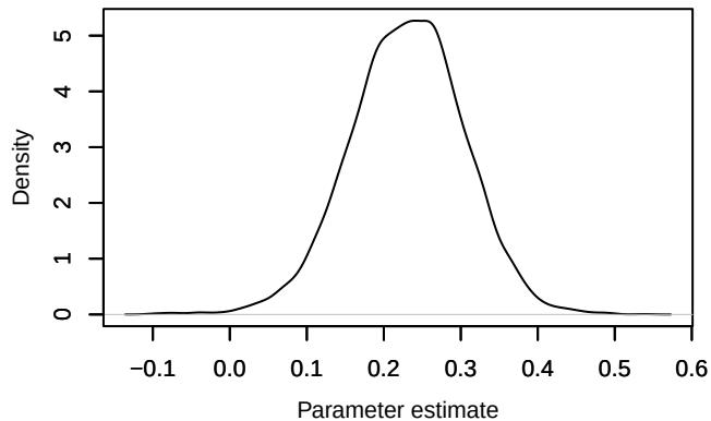
Density – \text{lp}[6, 1]
