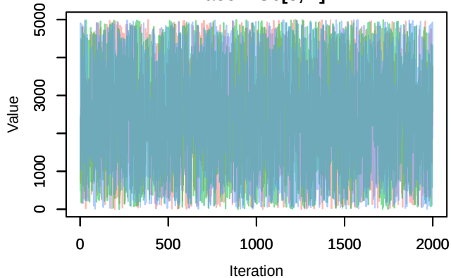
Trace – U0[4, 2]
