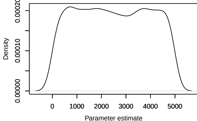
Density – U0[2, 2]
