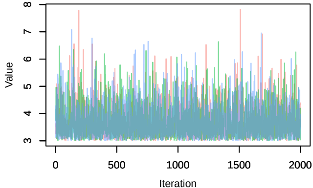
Trace – nu[2]
