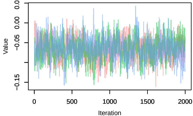
Trace – lp[1, 1]
