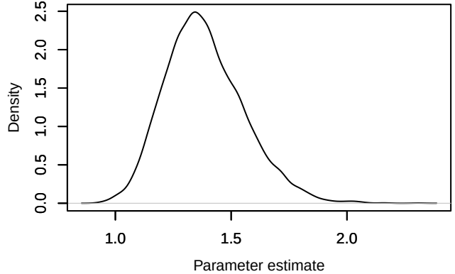
Density – sigma_phi[1]
