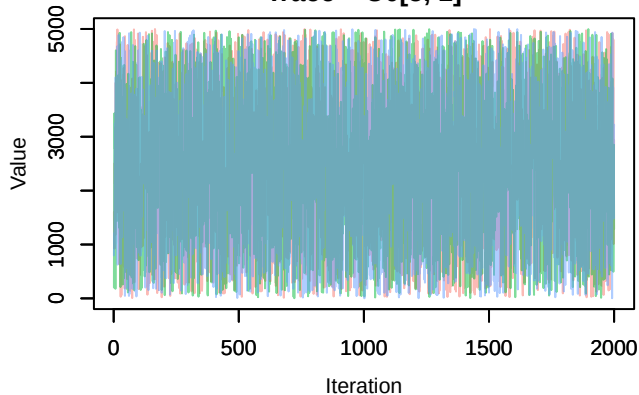
Trace – U0[6, 1]
