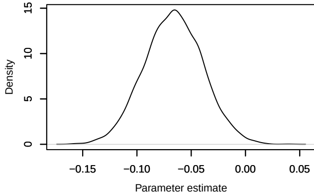
Density – lp[1, 1]
