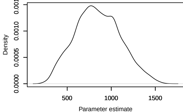
Density – U0[2, 1]
