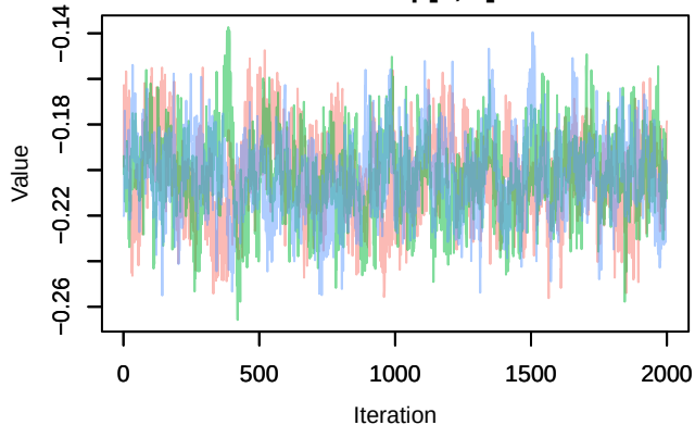
Trace – \text{lp}[6, 2]
