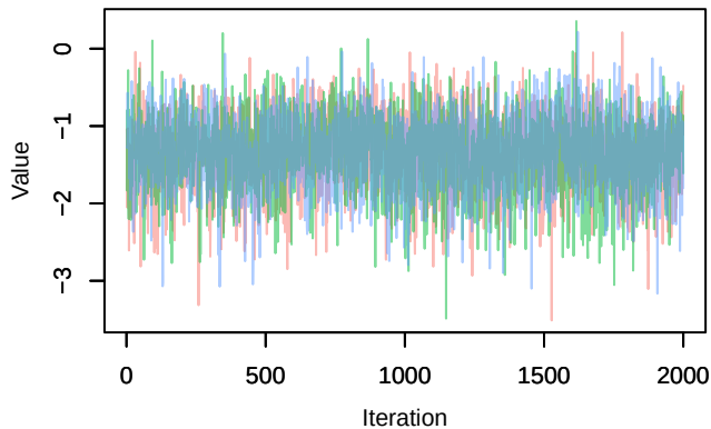
Trace – mu_r[2]
