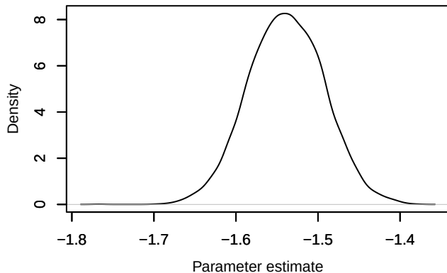
Density – \text{lp}[3, 1]
