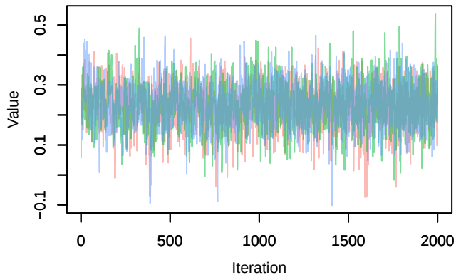
Trace – \text{lp}[6, 1]
