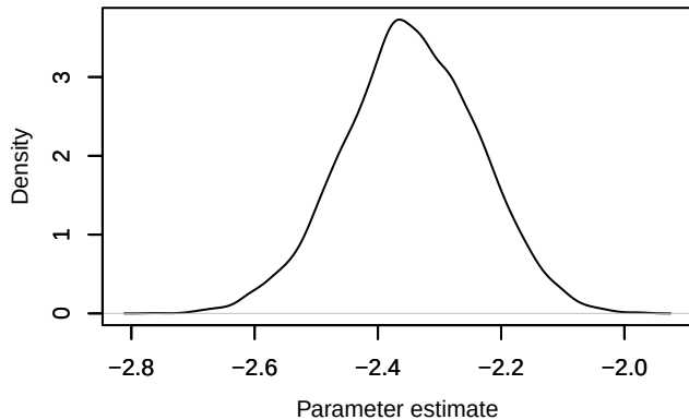
Density – \text{lp}[4, 1]
