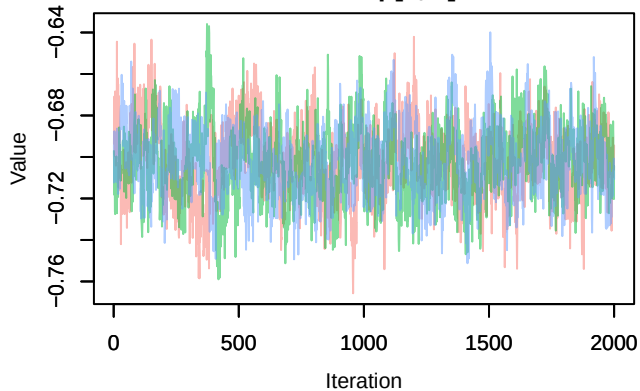
Trace – \text{lp}[5, 2]
