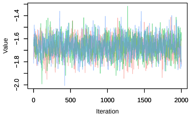
Trace – lpsi[2]
