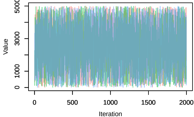
Trace – U0[3, 1]
