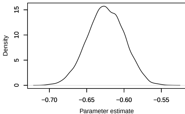
Density – \text{lp}[6, 2]
