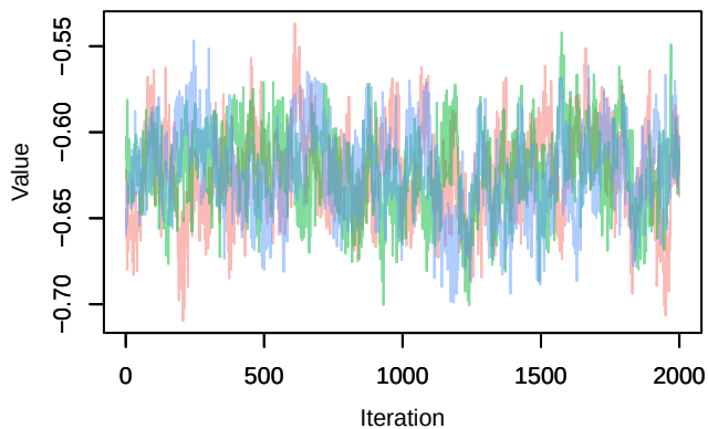
Trace – \text{lp}[6, 2]
