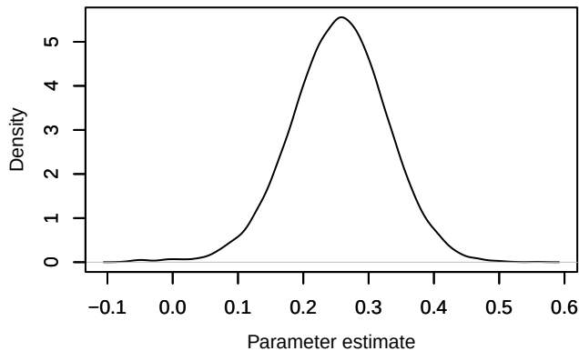
Density – \text{lp}[6, 1]
