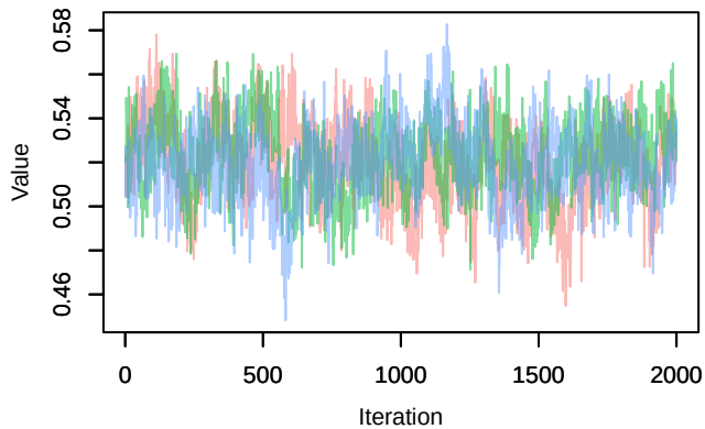
Trace – \text{lp}[3, 2]
