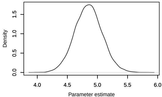
Density – mu_phi[2]
