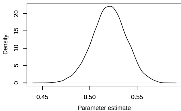
Density – \text{lp}[3, 2]
