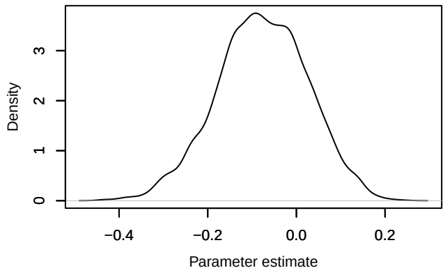
Density – \text{lp}[7, 1]
