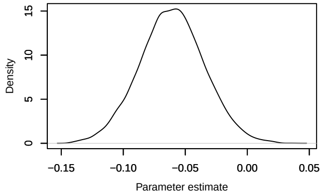
Density - lp[1, 1]
