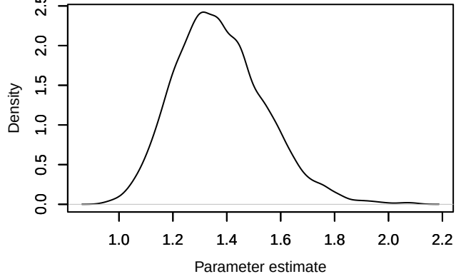
Density – sigma_phi[1]
