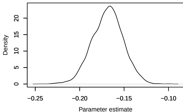
Density – \text{lp}[5, 2]
