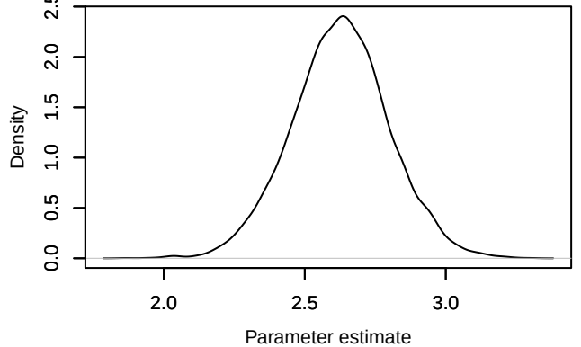
Density – sigma_phi[1]
