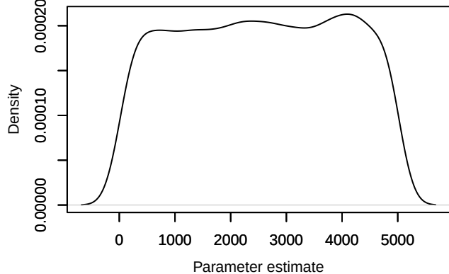
Density – U0[1, 1]
