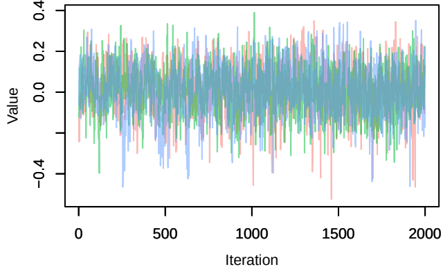
Trace – lp[2, 1]
