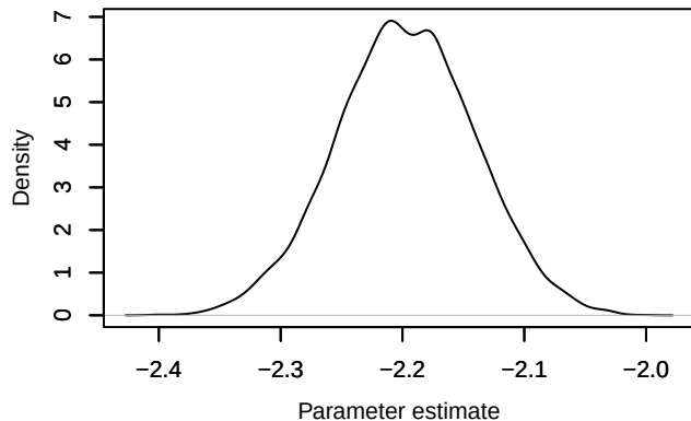
Density – lp[2, 1]
