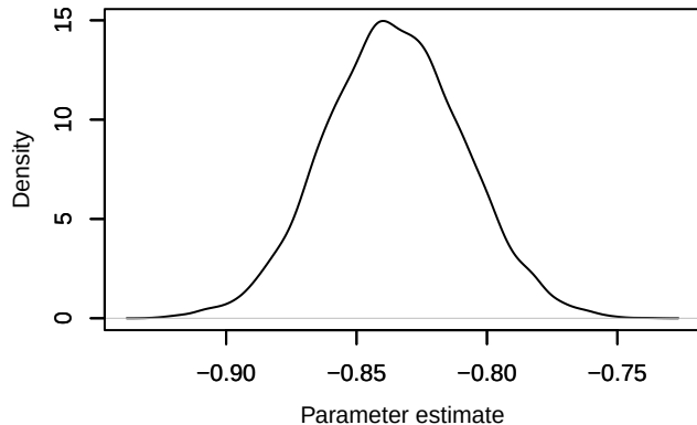
Density – \text{lp}[2, 2]
