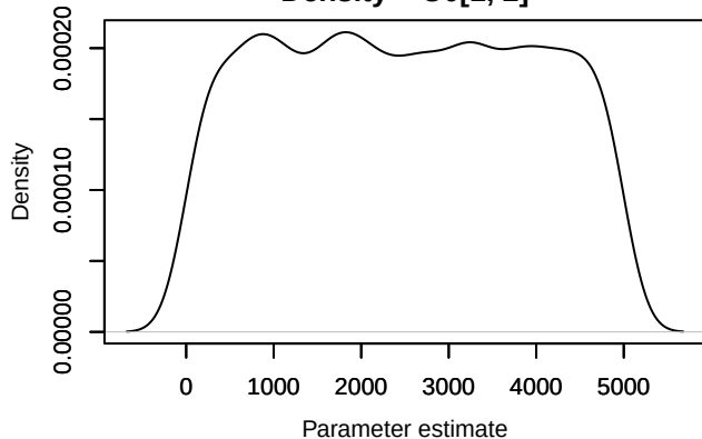
Density – U0[1, 2]
