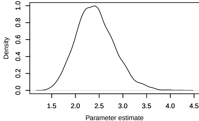
Density – nu[1]
