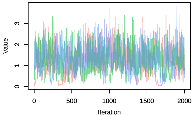
Trace – sigma_r[2]
