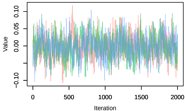
Trace – \text{lp}[1, 2]
