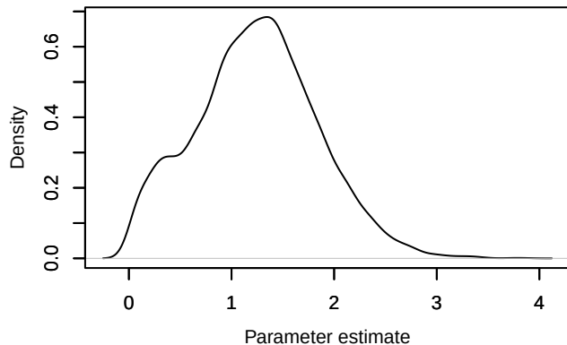
Density – sigma_r[2]
