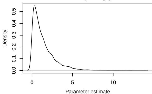
Density – nu[2]
