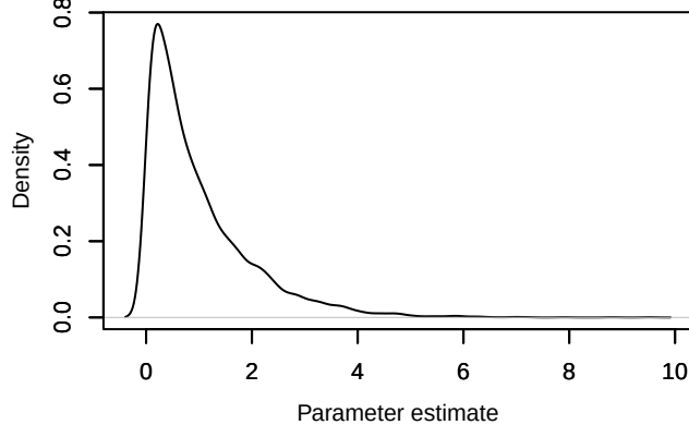
Density – U0[1, 1]
