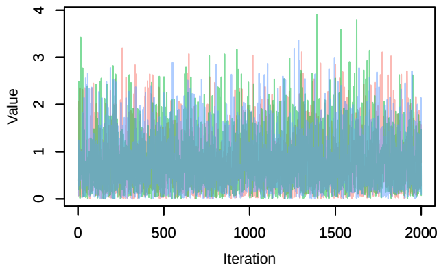
Trace – sigma_phi[2]
