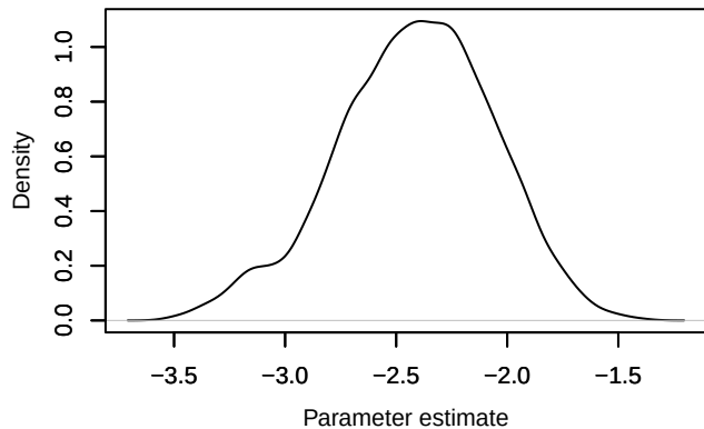
Density – IpsiLA[2]
