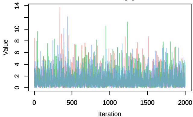
Trace – nu[2]
