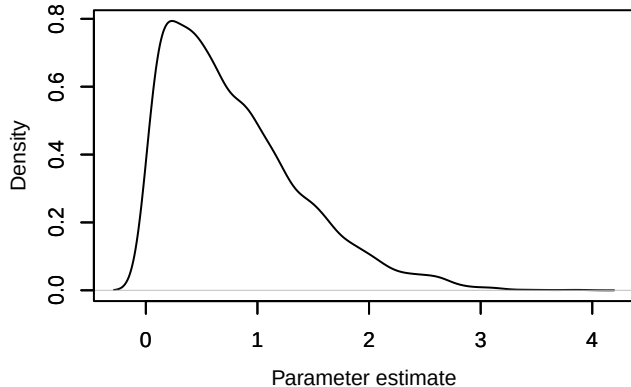
Density – sigma_phi[2]
