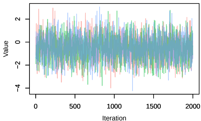
Trace – dJ[2]
