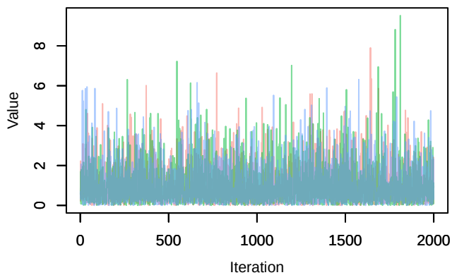
Trace – U0[1, 1]
