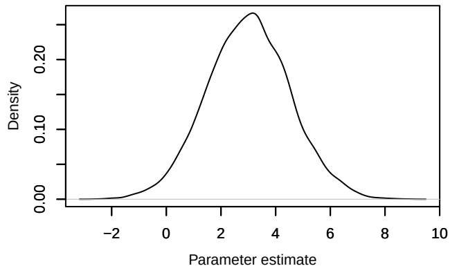
Density – sigma_phi[1]
