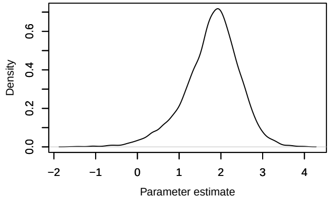
Density – mu_r[1]
