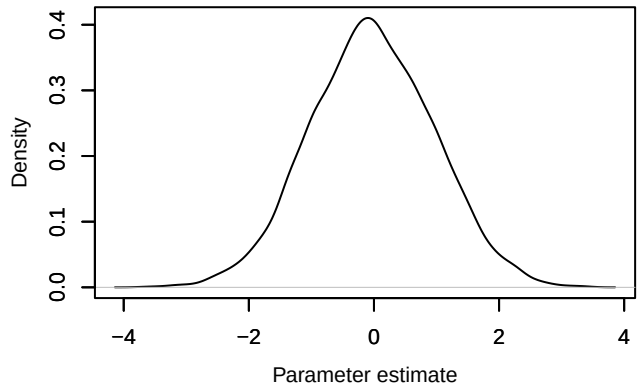
Density – mu_r[1]
