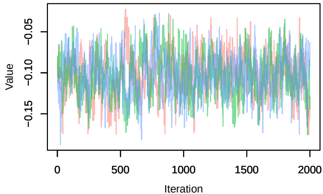
Trace – \text{lp}[1, 3]
