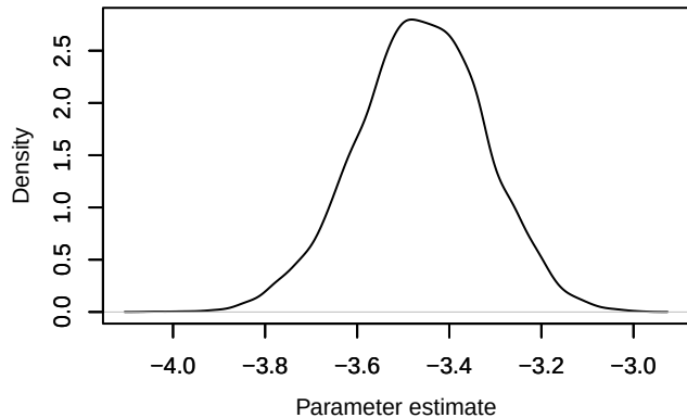
Density – a0[1]
