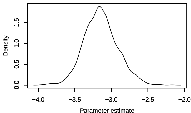
Density – dJ[1]
