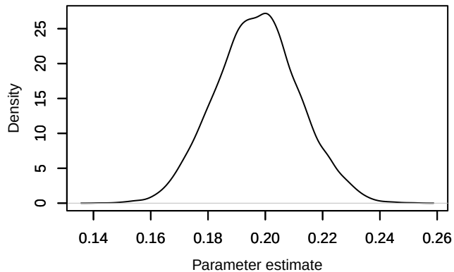
Density – g_eff[2]
