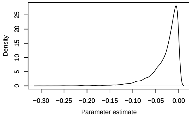
Density – dS[2]
