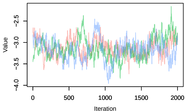
Trace – dJ[1]
