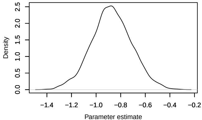
Density – b_post[2, 2]
