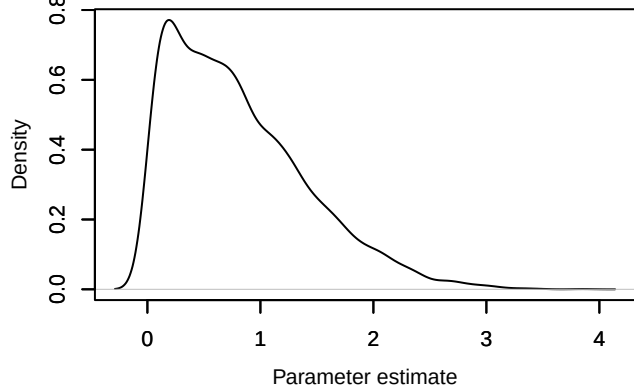
Density – sigma_r[2]
