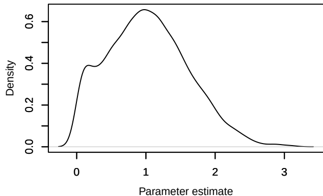
Density – sigma_r[2]
