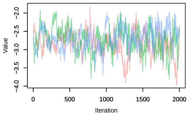
Trace – b_postJ[1, 1]
