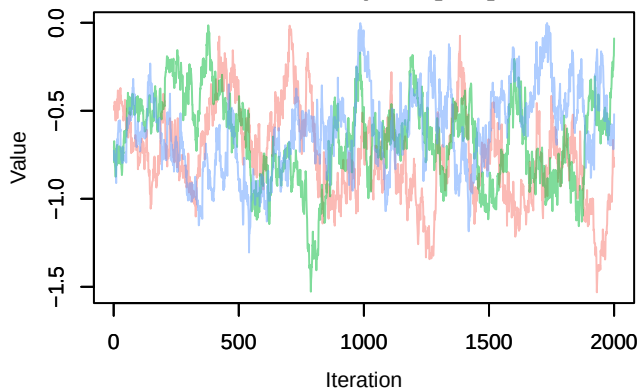
Trace – b_postJ[2, 2]
