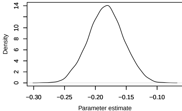
Density – lp[1, 2]
