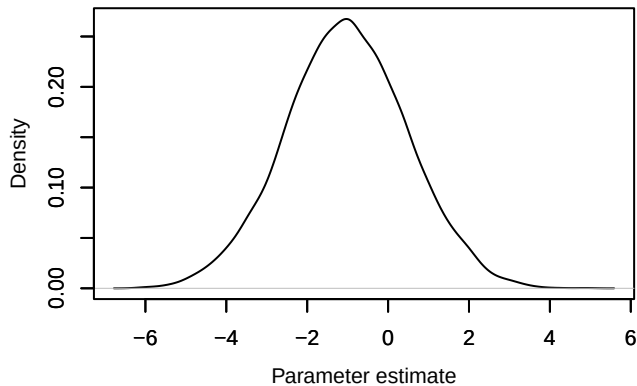
Density – a1[1]
