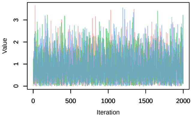
Trace – dJ[1]
