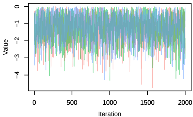
Trace – b_postJ[2, 1]
