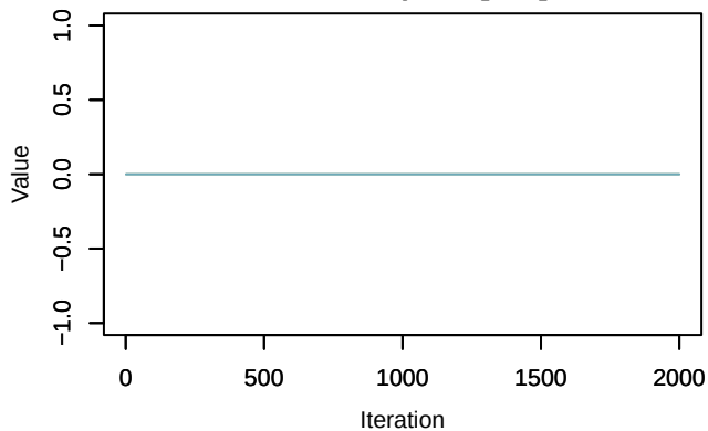
Trace – lpsiSL[1]
