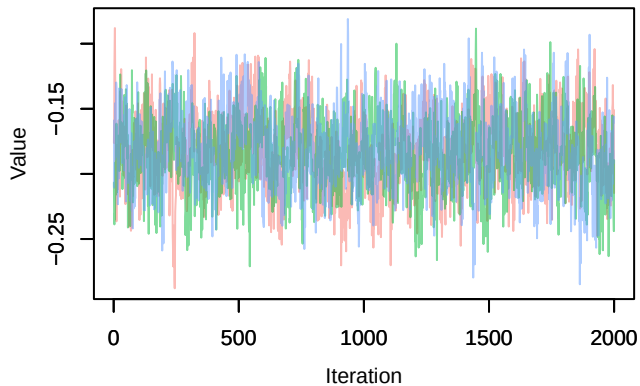
Trace – lp[1, 2]
