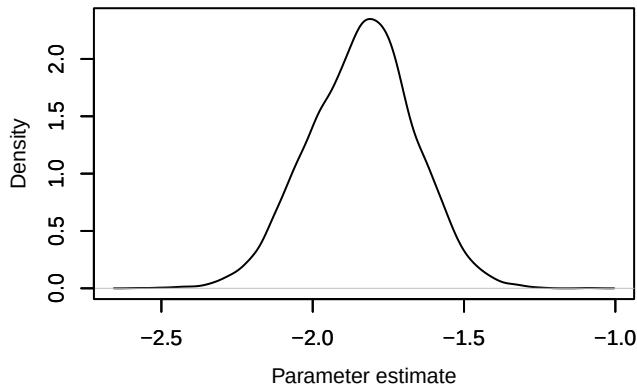
Density – a1[2]
