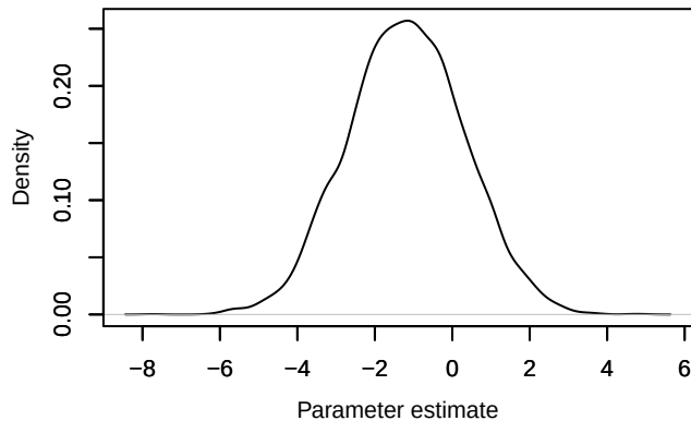
Density – sigma_r[1]
