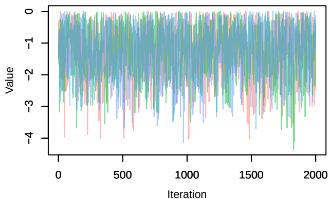
Trace – b_postJ[2, 2]
