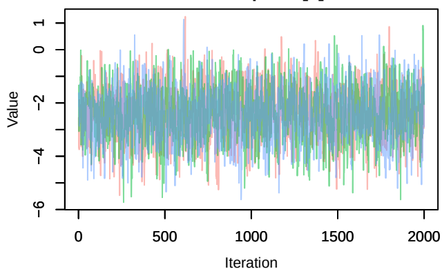
Trace – lpsiSL[2]
