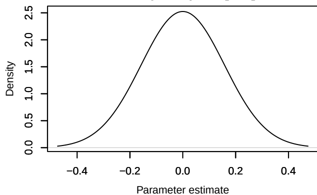
Density – lpsiSL[1]
