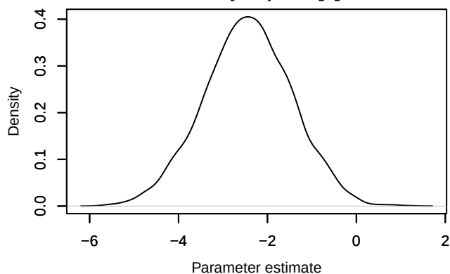
Density – lpsiSL[2]
