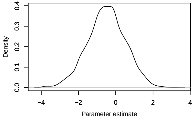
Density – dJ[2]
