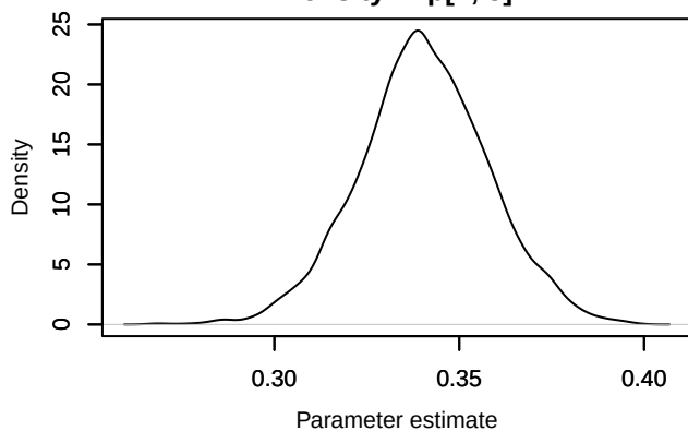
Density – \text{lp}[3, 3]
