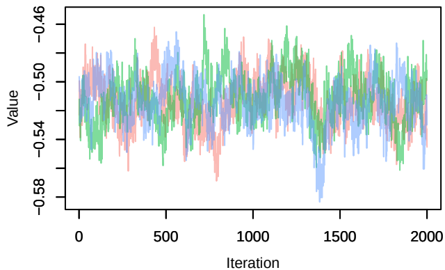
Trace – \text{lp}[1, 3]
