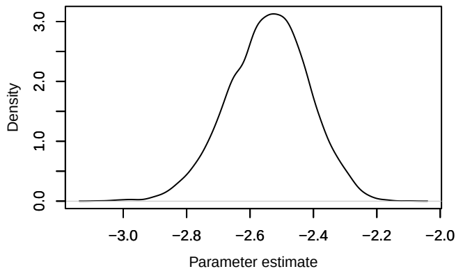
Density – \text{lp}[4, 2]
