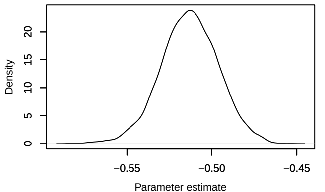
Density – \text{lp}[1, 3]
