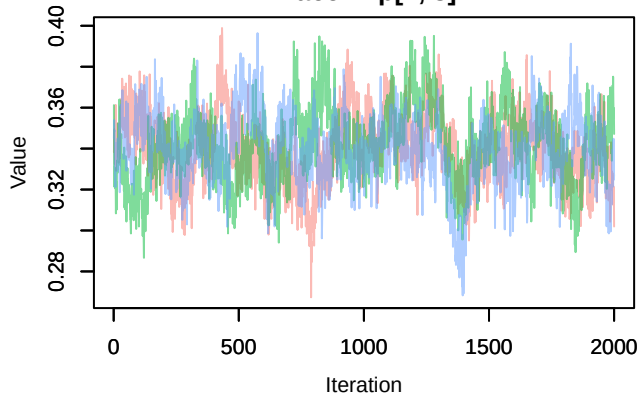
Trace – \text{lp}[3, 3]
