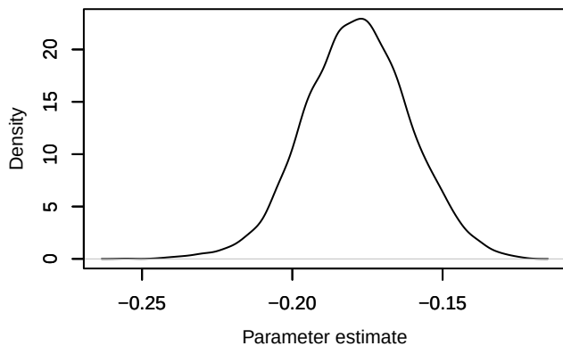
Density – \text{lp}[4, 3]
