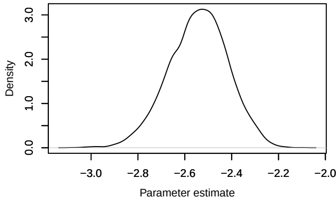
Density – \text{lp}[3, 1]
