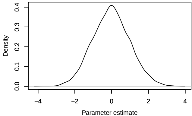
Density – mu_r[1]
