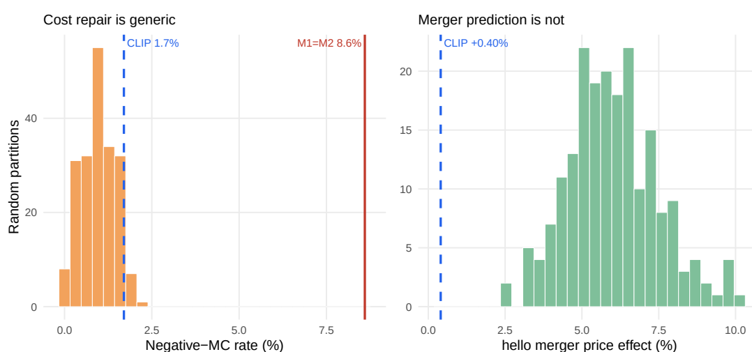
Figure 5.2: Placebo nesting tests (200 random cross-firm partitions). Left: the negative-MC rate under random nests (bars) reaches CLIP’s level (blue dashed) or lower in 96% of draws – the cost-side repair is generic, far below the M1=M2 baseline (red). Right: the simulated hello merger price effect under random nests ranges from +2.5% to +10.2%; CLIP’s +0.40% (blue dashed) lies below all 200 draws, because CLIP alone keeps Colgate’s product line out of hello’s nest.
