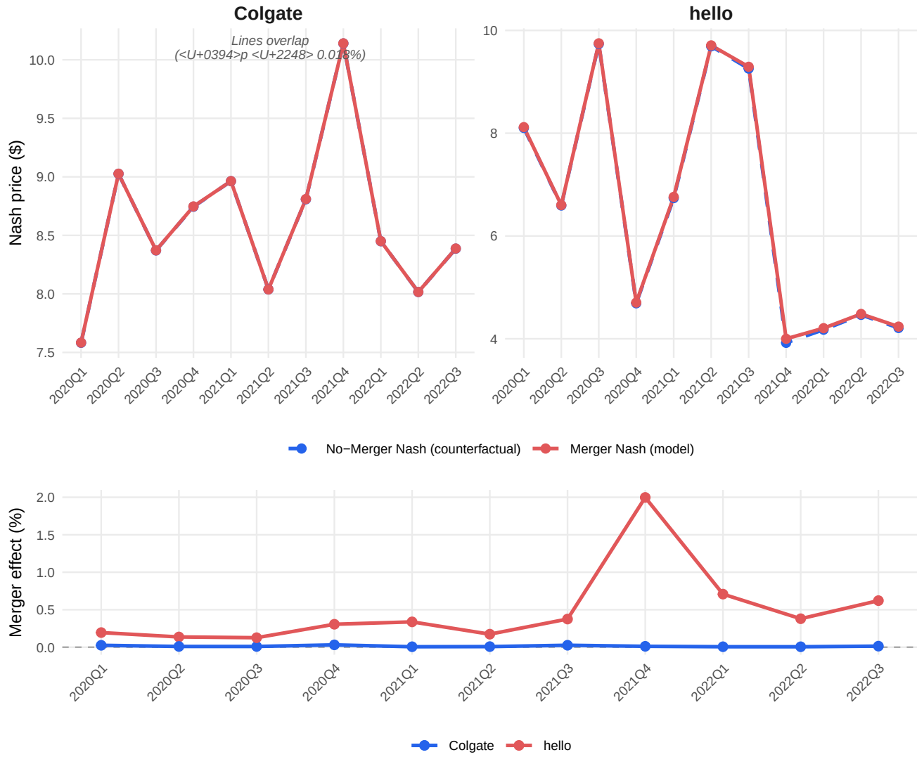
Figure 5.1: Merger simulation price trajectories (Model 3, CLIP-Nested, \rho^* = 0.67 ).
