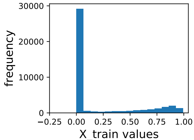
hist. for feature 224
