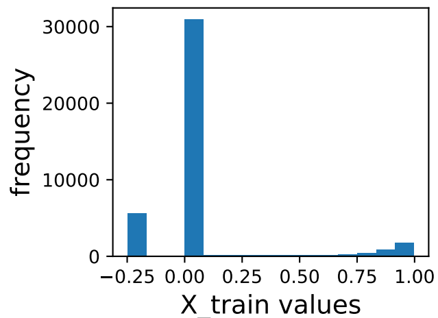
hist. for feature 114
