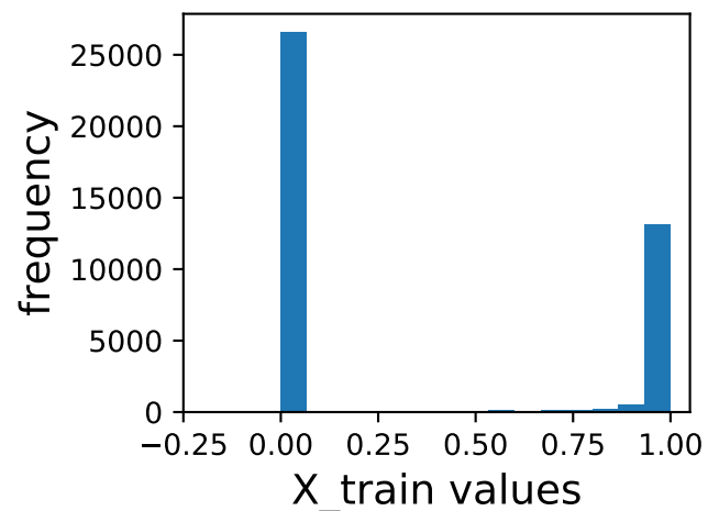
hist. for feature 283
