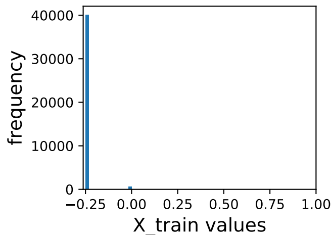
hist. for feature 175
