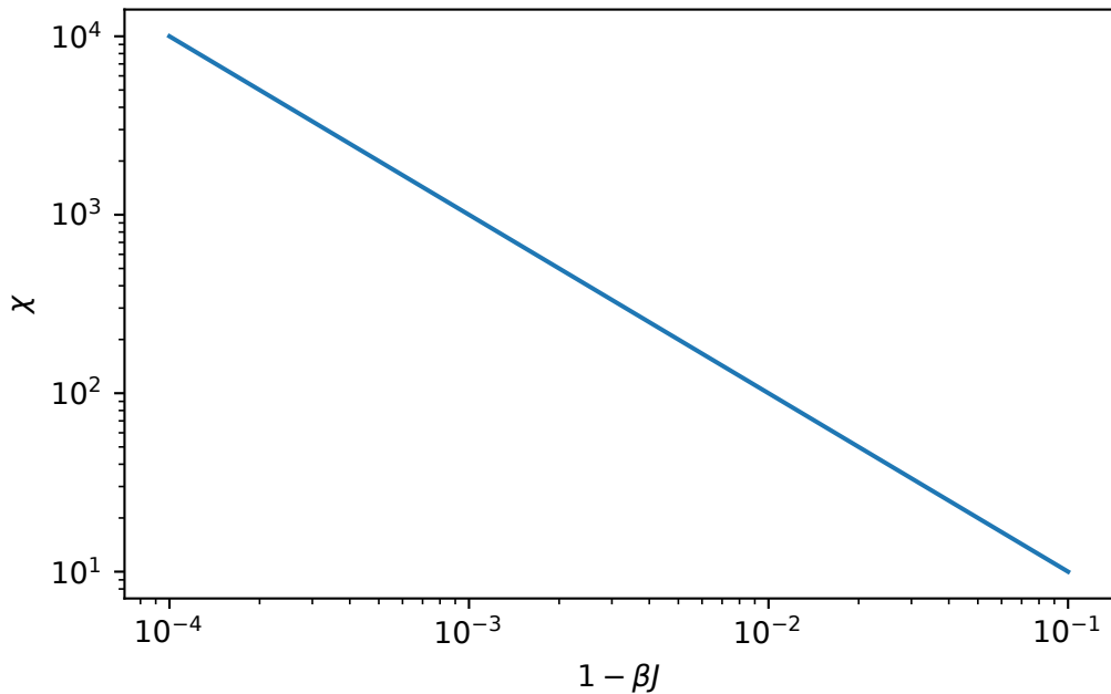
Susceptibility, fitted \gamma = 1.000 (exact 1)
