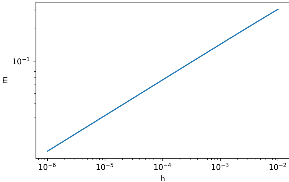
Critical isotherm, fitted \delta = 3.004 (exact 3)
