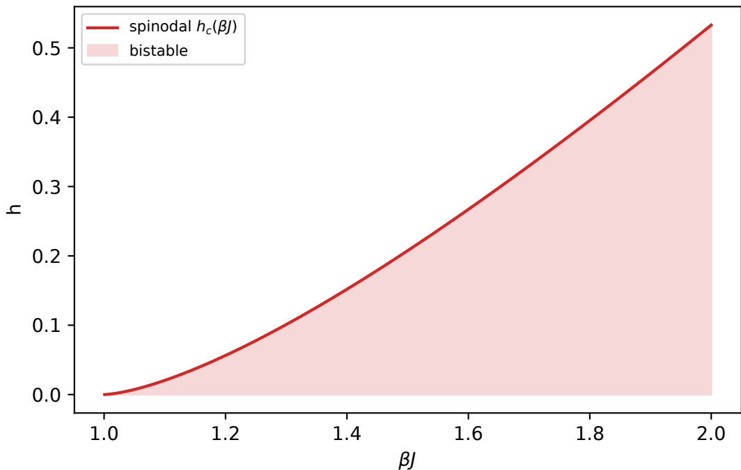
Phase diagram: where two opinions coexist
