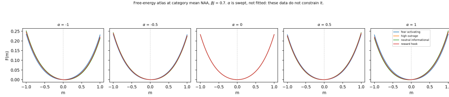
Figure 5: Free energy swept across a range of couplings, evaluated at each category’s measured mean. The sweep is not a fit: no value of \alpha is estimated from the data anywhere in this paper, and the panels show how the physics would behave for each coupling rather than which coupling holds.
