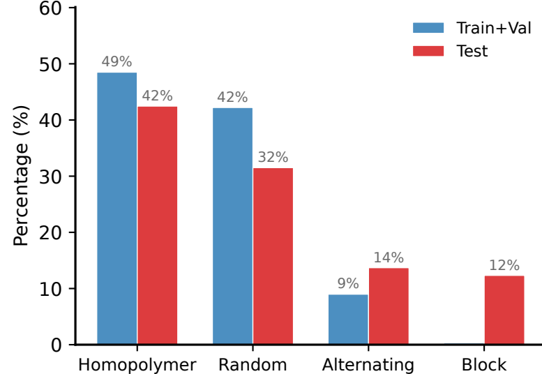
Copolymer Architecture
