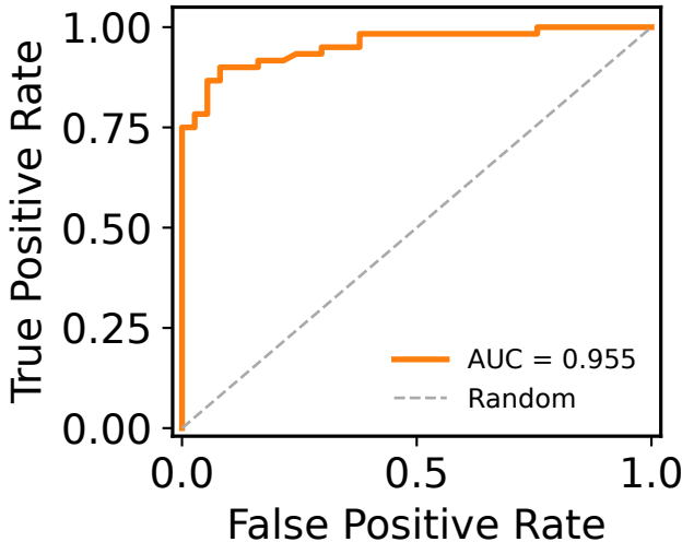
ROC — XGB (FP+pooled poly)
