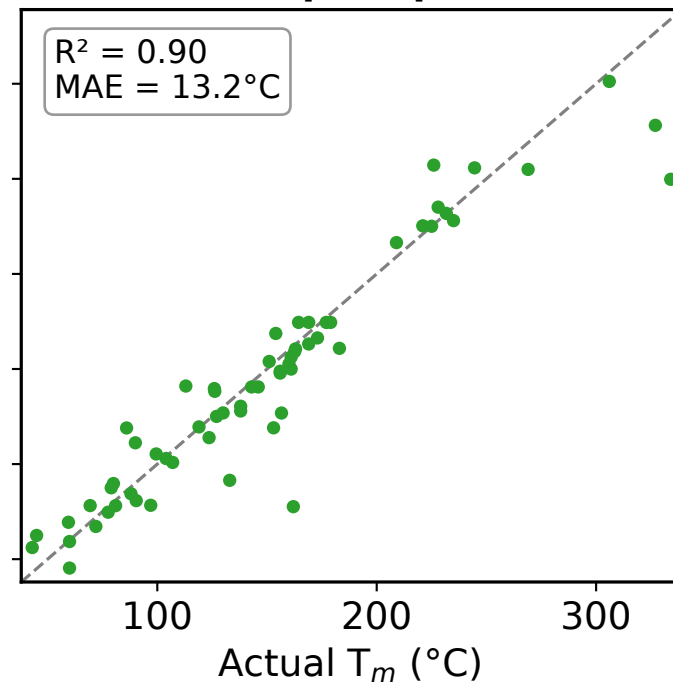
XGB (RepFP+pooled)
