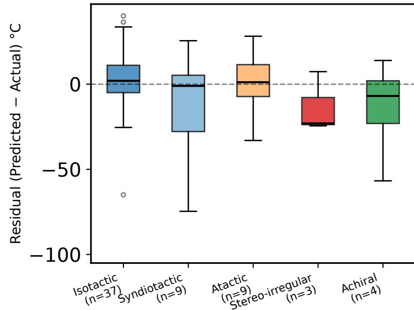
GATv2 (PBG)
