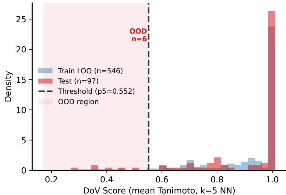
Domain of Validity Distribution
