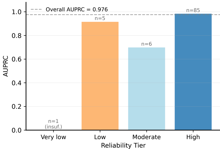
Classifier Performance by DoV Tier (XGB FP POOLED POLY)
