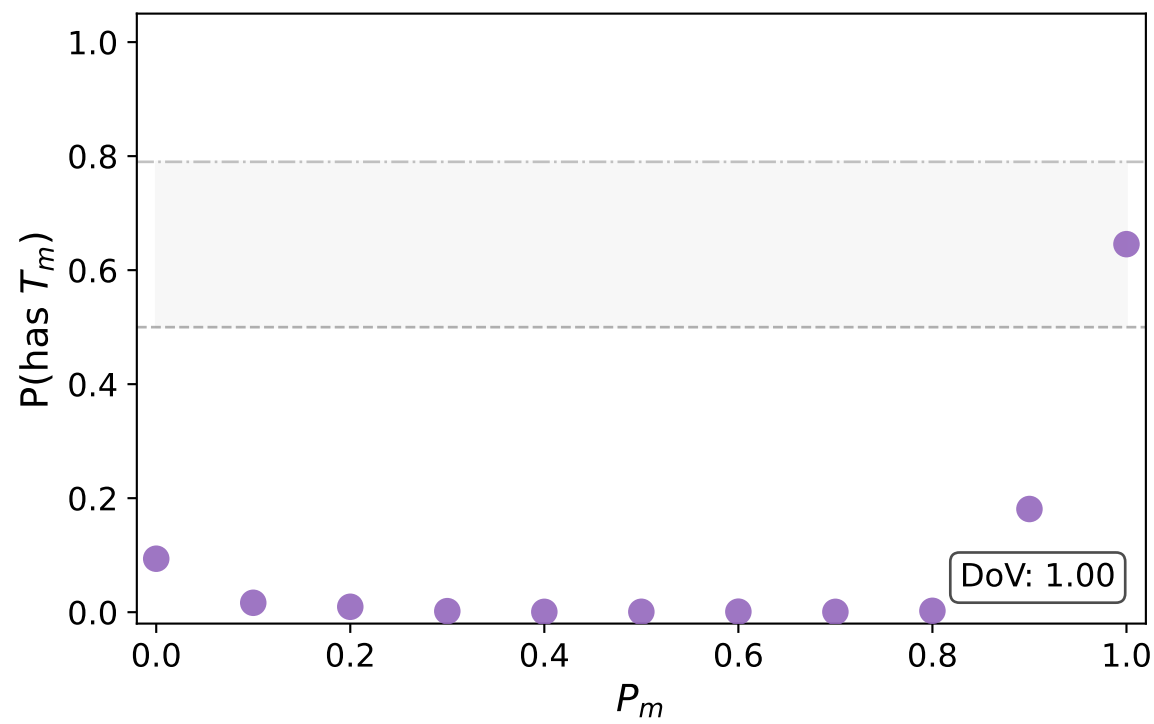
PNIPAM
