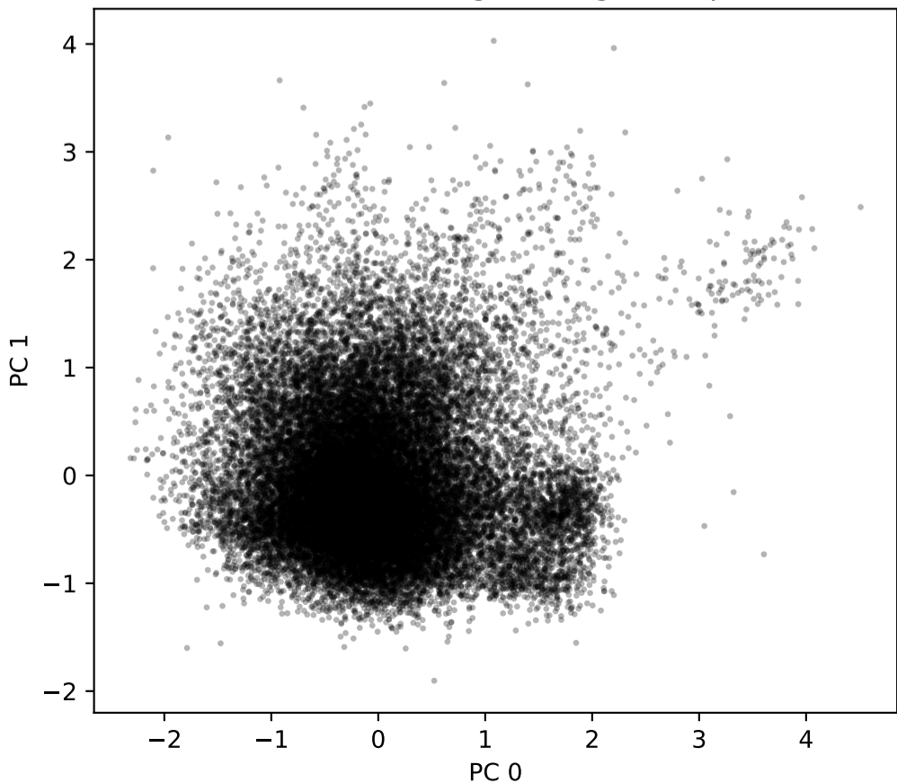
PCA of latent encoding of cell gene expression
