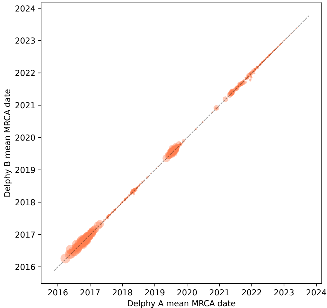
Clade MRCA dates (883 clades present in both)
