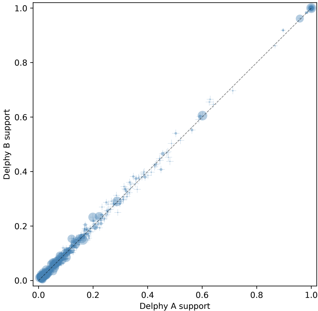
Clade posterior support (ESS: Delphy A=1354, Delphy B=1295)
