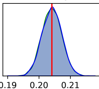
HKY \pi_C
