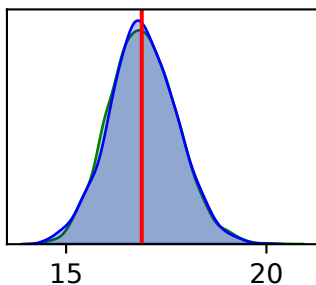
HKY \kappa
