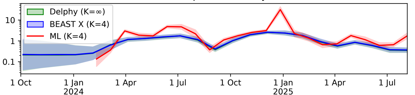
Effective Population Size (years)
