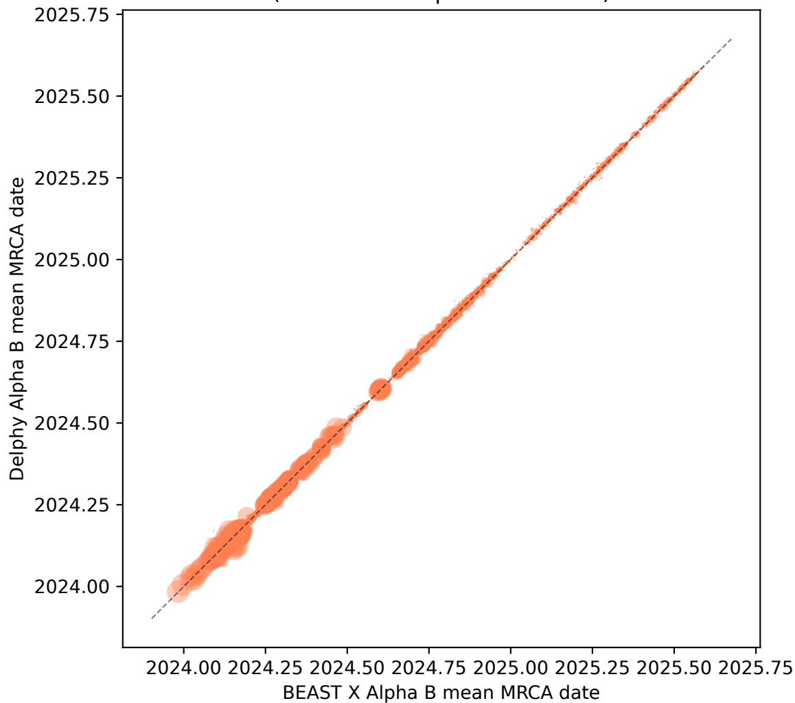
Clade MRCA dates (42014 clades present in both)
