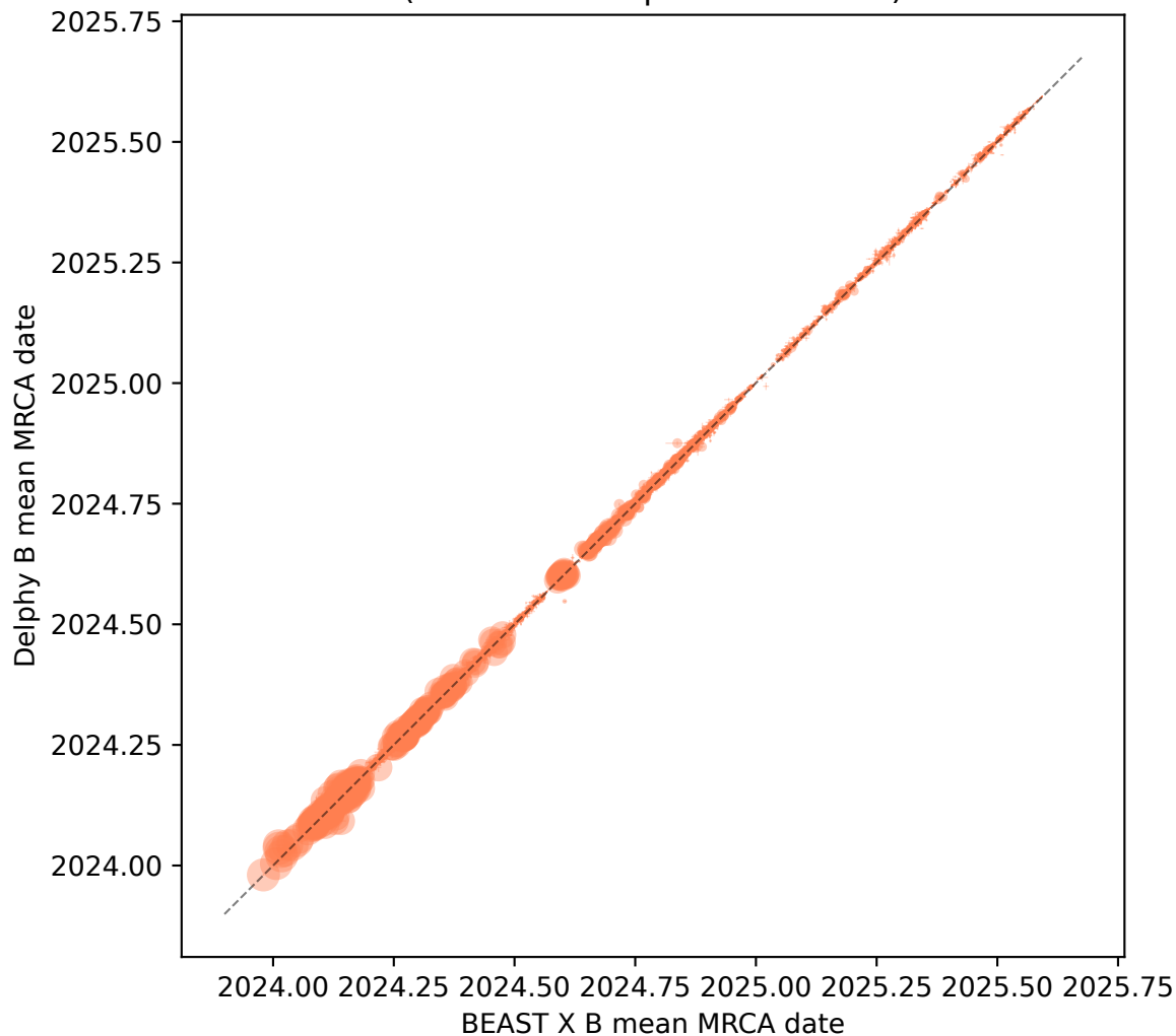
Clade MRCA dates (41664 clades present in both)
