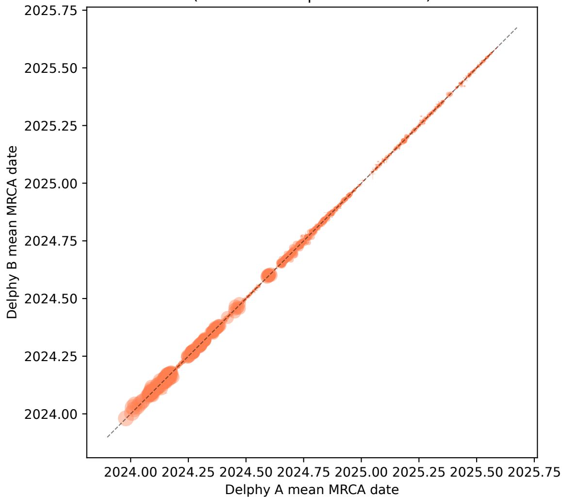
Clade MRCA dates (38452 clades present in both)
