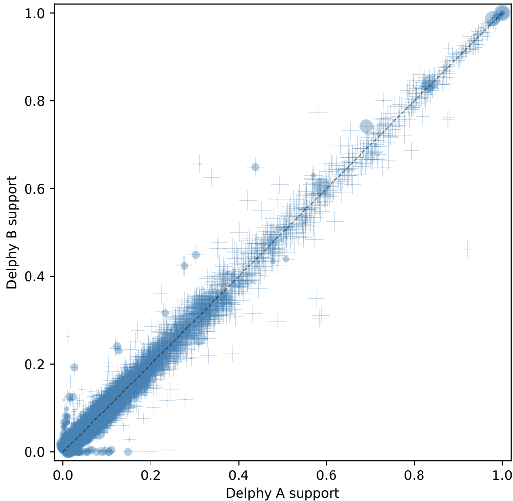
Clade posterior support (ESS: Delphy A=581, Delphy B=481)
