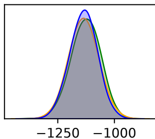
Coalescent Prior
