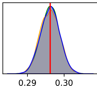
HKY \pi_A
