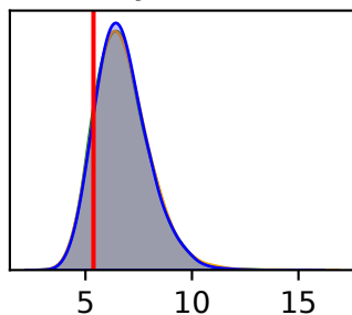
Final Pop Size (years)
