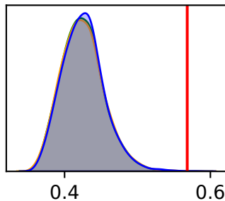
Tree Height (years)
