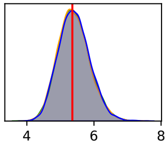
HKY \kappa
