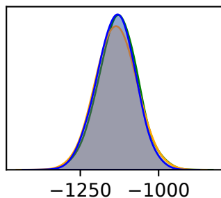
Coalescent Prior
