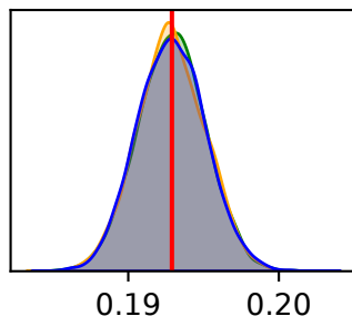
Pop Growth Rate (1/year)
