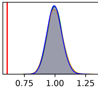
Mutation rate ( \times 10^{-3} /site/year)
