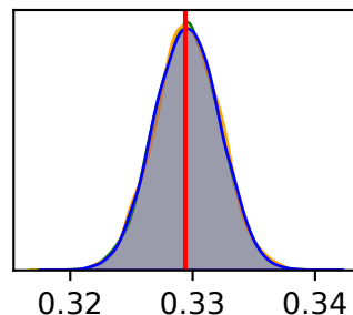
HKY \pi_T
