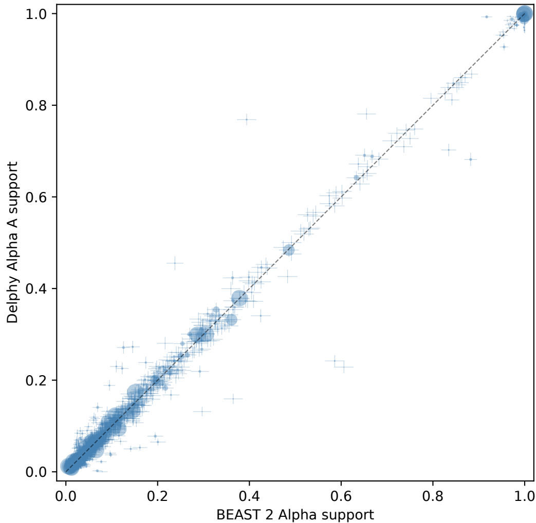
Clade posterior support (ESS: BEAST 2 Alpha=530, Delphy Alpha A=1083)
