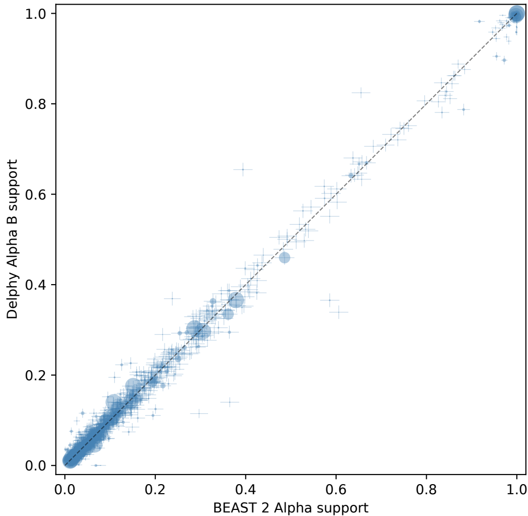
Clade posterior support (ESS: BEAST 2 Alpha=530, Delphy Alpha B=1002)
