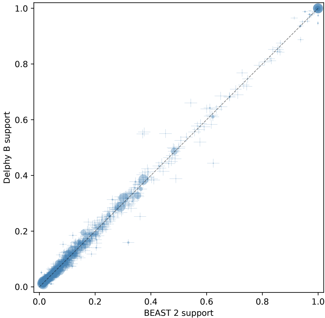
Clade posterior support (ESS: BEAST 2=480, Delphy B=988)
