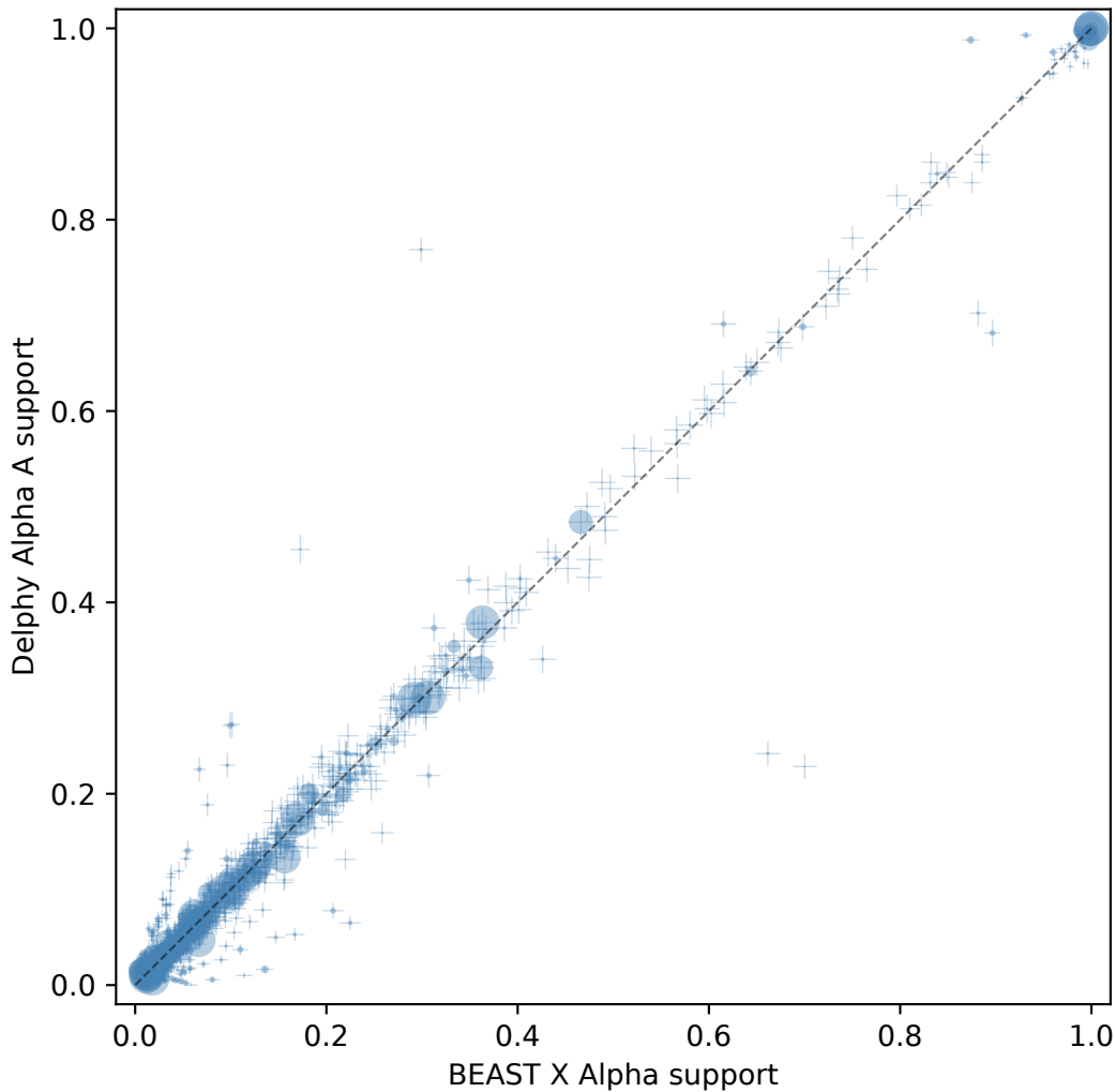
Clade posterior support (ESS: BEAST X Alpha=1347, Delphy Alpha A=1083)
