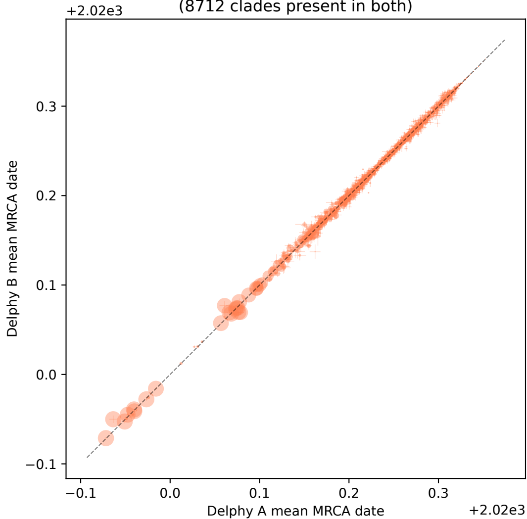
Clade MRCA dates (8712 clades present in both)
