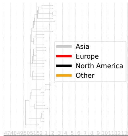
Epiweek 2020-06 (N=1023) (ending on 8 Feb 2020)
