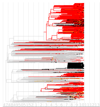
Epiweek 2020-10 (N=5584) (ending on 7 Mar 2020)
