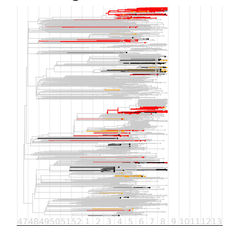
Epiweek 2020-08 (N=1662) (ending on 22 Feb 2020)
