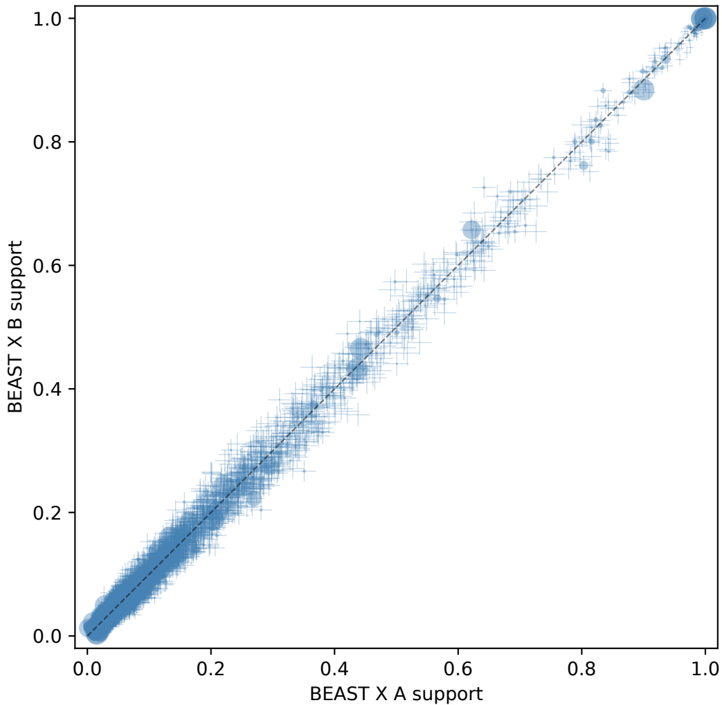
Clade posterior support (ESS: BEAST X A=652, BEAST X B=641)
