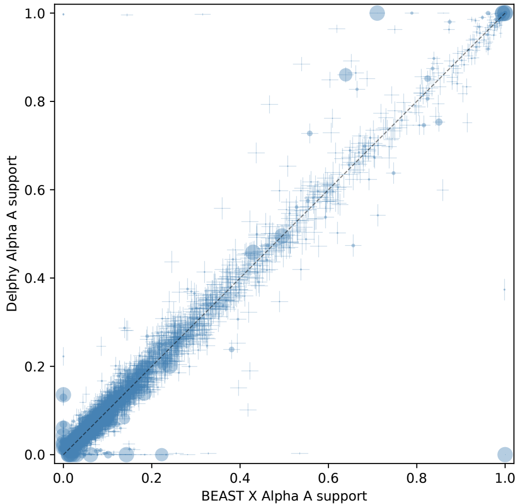
Clade posterior support (ESS: BEAST X Alpha A=653, Delphy Alpha A=392)
