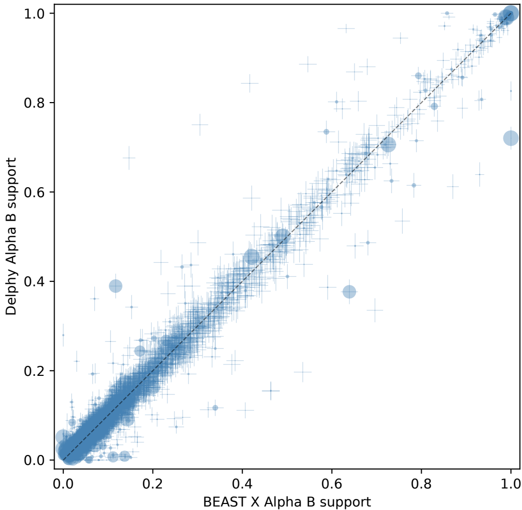
Clade posterior support (ESS: BEAST X Alpha B=630, Delphy Alpha B=309)
