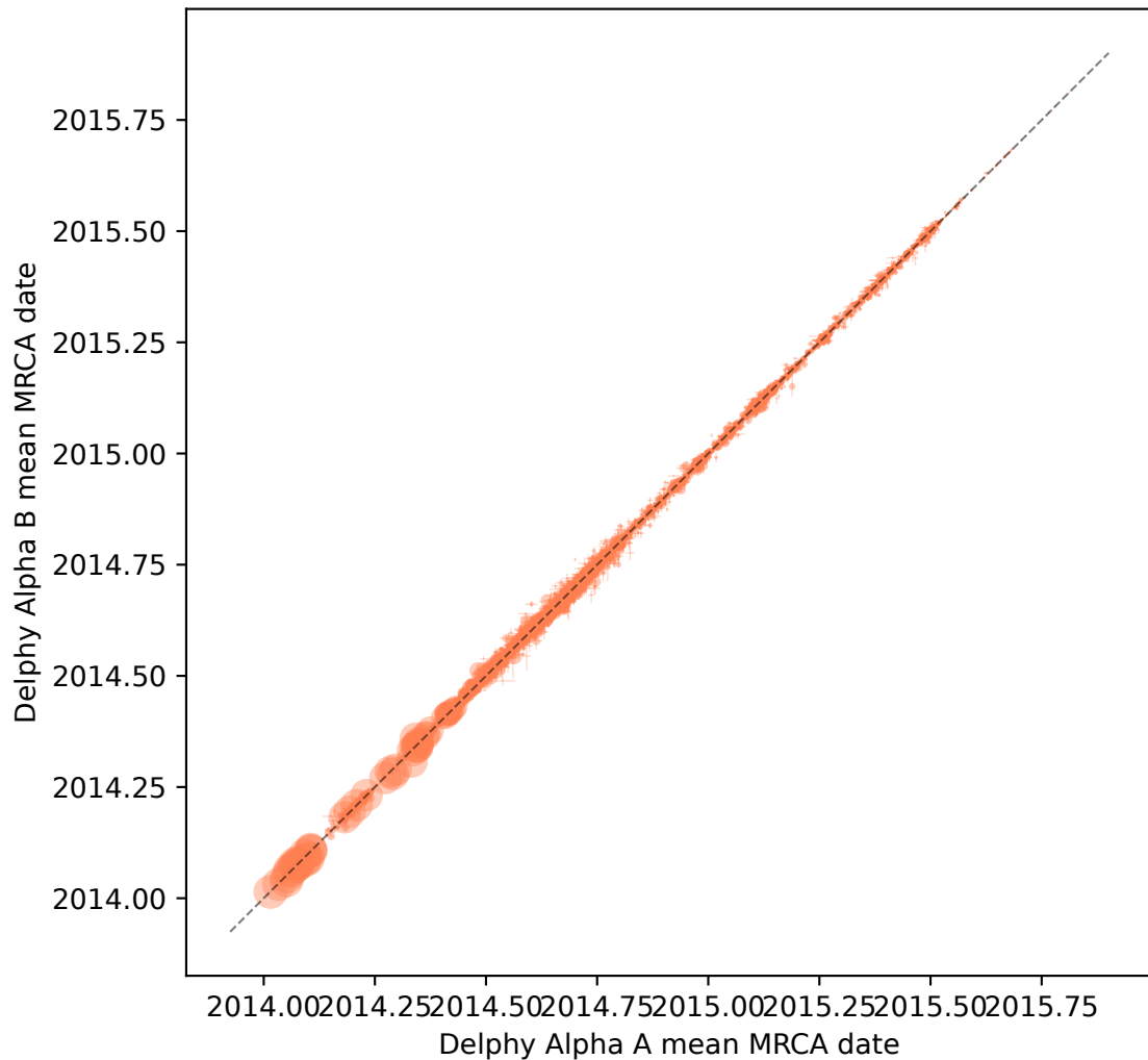
Clade MRCA dates (16562 clades present in both)
