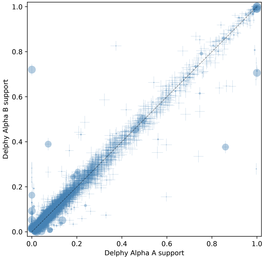
Clade posterior support (ESS: Delphy Alpha A=392, Delphy Alpha B=309)
