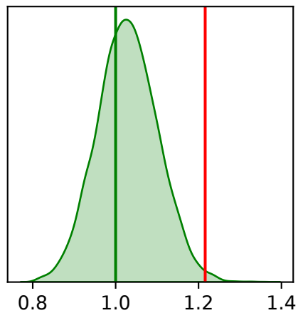
HKY \pi_A
