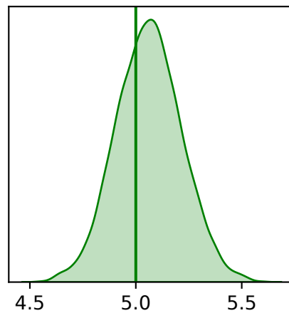
HKY \pi_G
