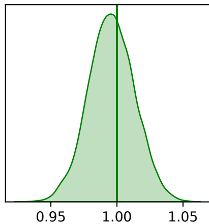
HKY \pi_A
