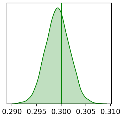
Coalescent Prior
