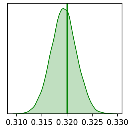
HKY \pi_T
