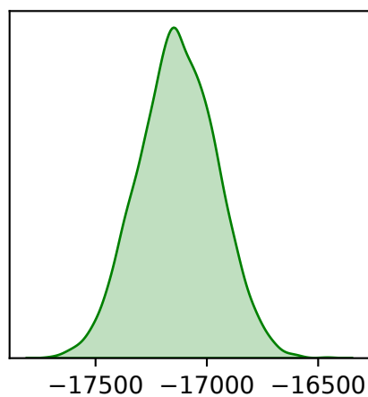
Coalescent Prior
