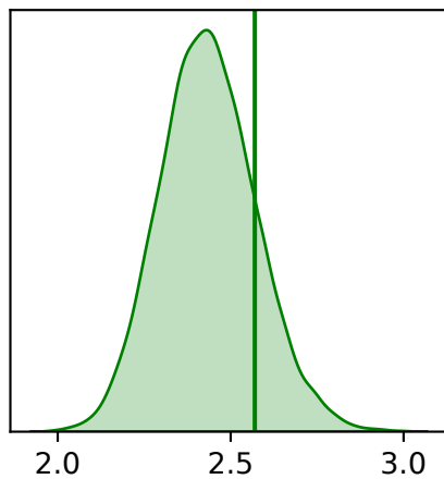
HKY \pi_C
