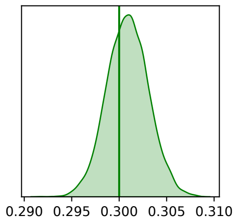
Coalescent Prior
