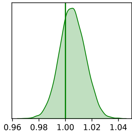
HKY \pi_A
