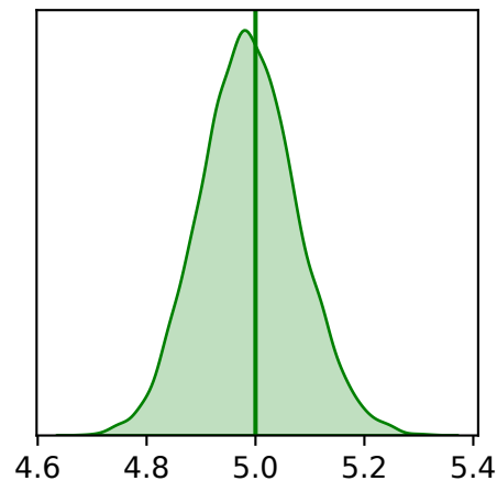
HKY \pi_G
