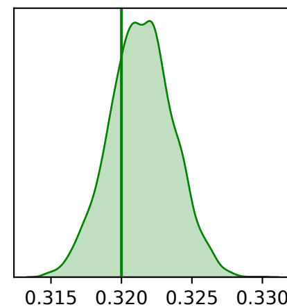
HKY \pi_T
