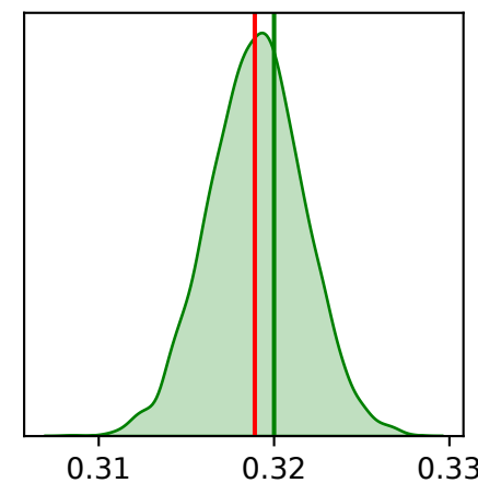
HKY \pi_T
