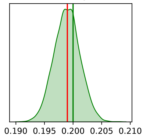
Pop Growth Rate (1/year)
