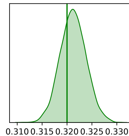
HKY \pi_T
