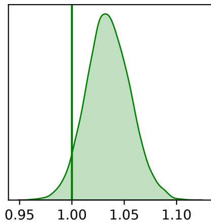
HKY \pi_A
