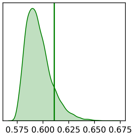
HKY \pi_C
