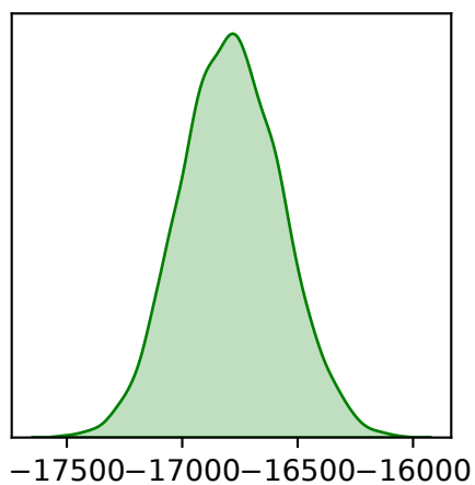
Coalescent Prior
