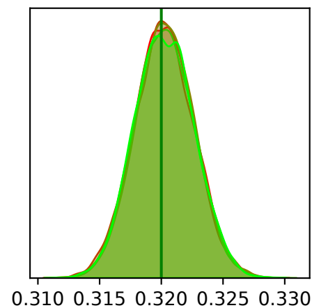
HKY \pi_T
