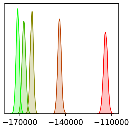
Coalescent Prior
