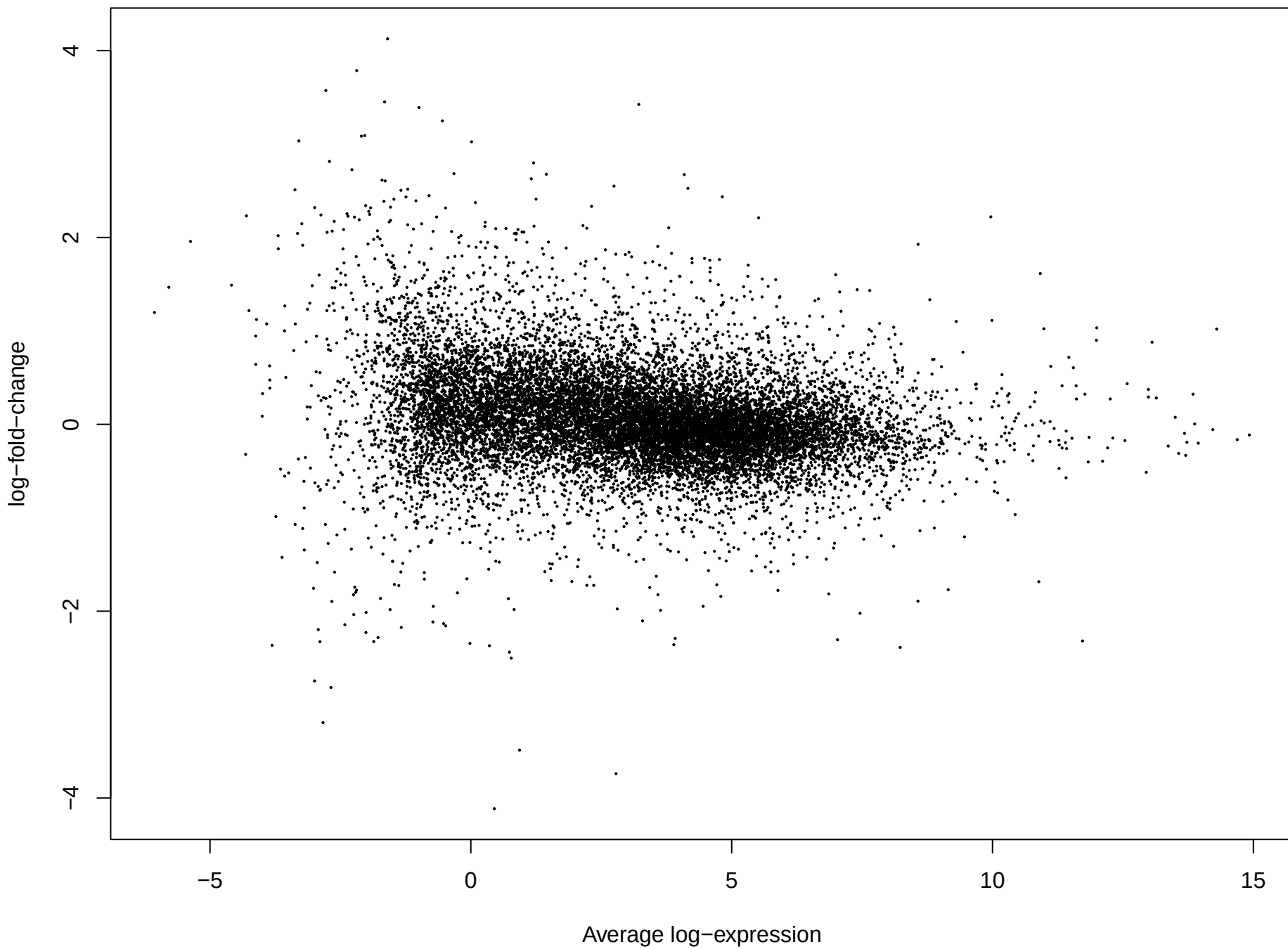
MA Plot
