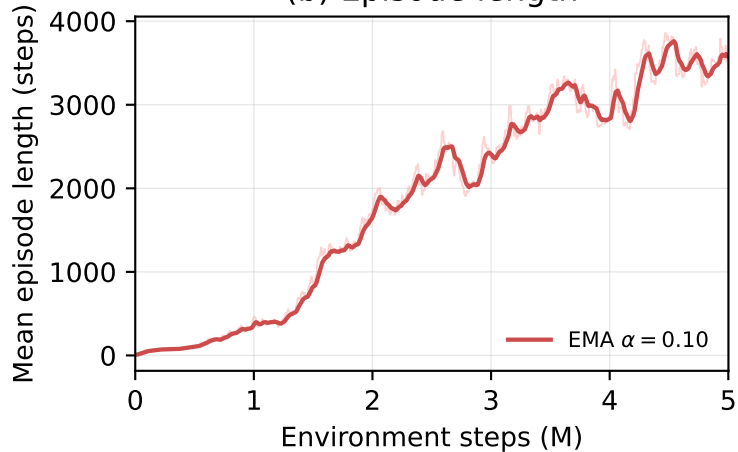
(b) Episode length
