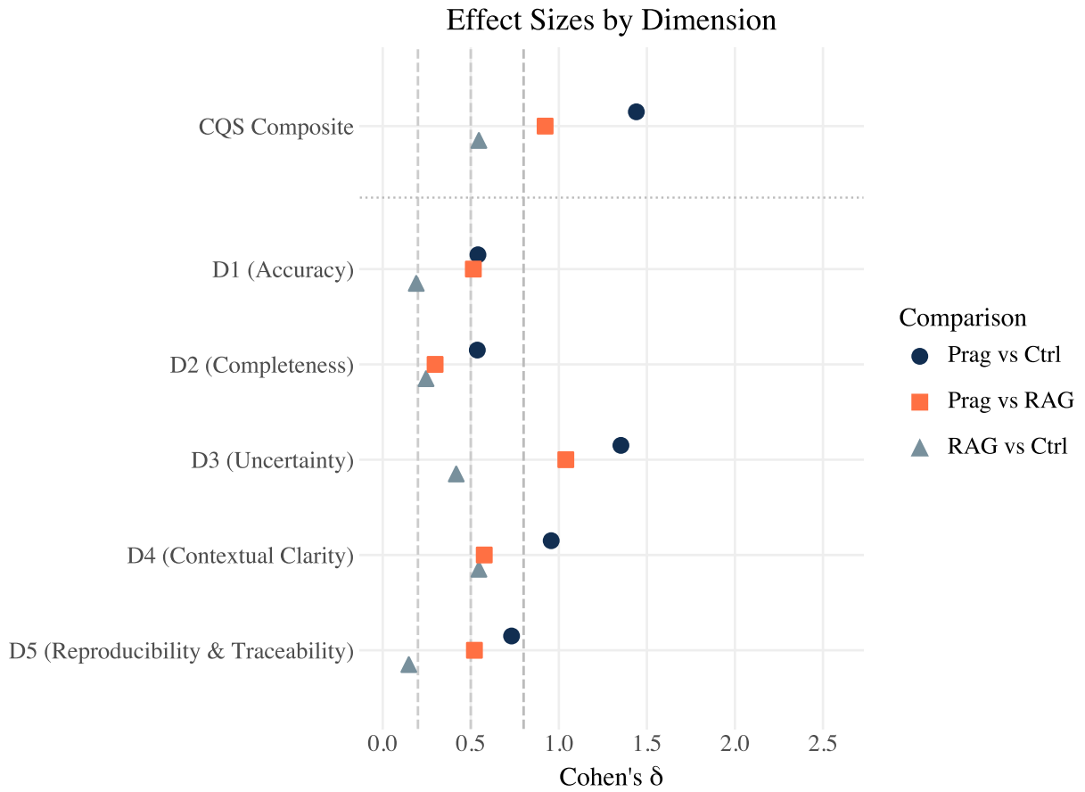
Figure 8: Cohen's d effect sizes by dimension. Vertical lines: d = 0.2 (small), 0.5 (medium), 0.8 (large).
