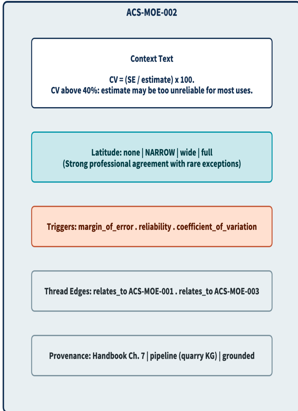
Figure 4: Anatomy of a pragmatic, showing the five structural components using ACS-MOE-002 (coefficient of variation threshold) as an example.
