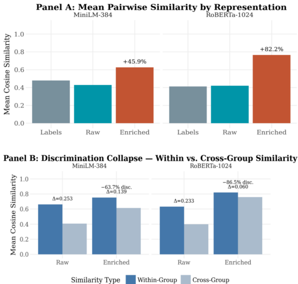
Figure 1: Semantic smearing in federal statistical metadata. Panel A: mean pairwise similarity increases with enrichment. Panel B: group discrimination collapses as within-group and cross-group similarity converge.
