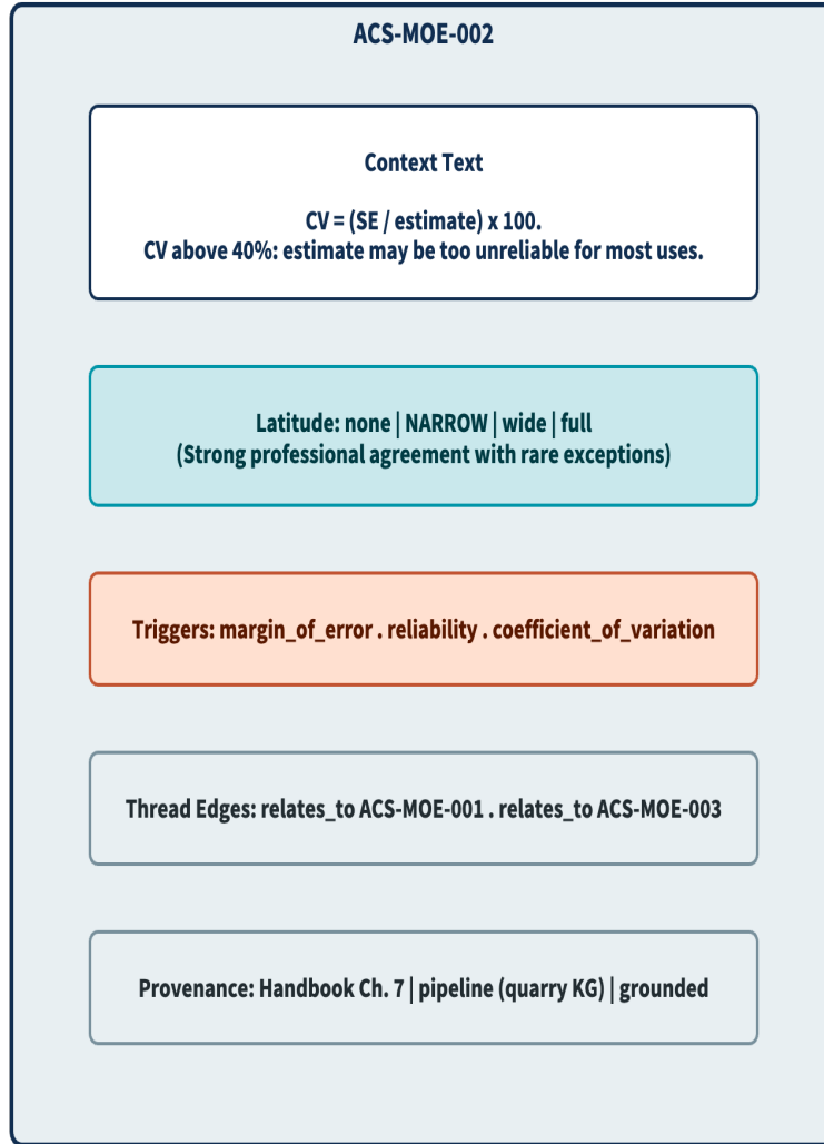
Figure 3: Anatomy of a pragmatic, showing the five structural components using ACS-MOE-002 (coefficient of variation threshold) as an example.
